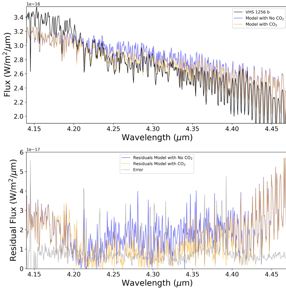
Figure 7. The JWST/NIRSpec spectrum of VHS 1256 b compared to two atmospheric models that contain CO 2 (orange) and a model with no opacity from CO 2 (blue). The data show excess absorption at 4.2 \mu\text{m} , which shows evidence of CO 2 absorption. The bottom panel shows residuals between the data and the models with the error plotted in gray. No CO 2 shows a larger residual than a model including the opacity of the molecule.
