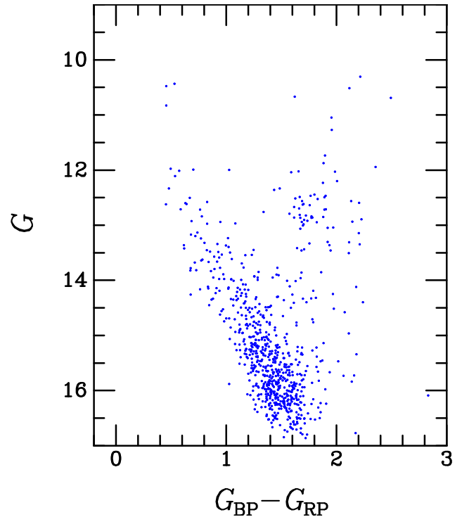
Figure 21. Color-magnitude diagram for a sample of stars in the Galactic disk at similar distances to that of the black hole, selected from Gaia EDR3 as described in the text. The population at this location contains main-sequence stars of a younger population, and older stars with redder colors.
