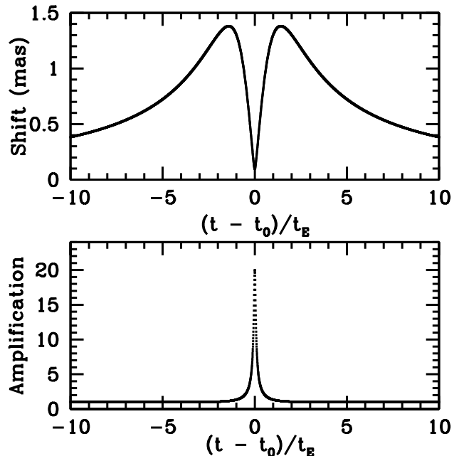
Figure 2. Astrometric shift (top panel) and light magnification (bottom panel) for a microlensing event produced by a 5 M_\odot black hole at a distance of 2 kpc passing in front of a background star at 8 kpc. The assumed minimum impact parameter is u_0 = 0.05 . The maximum astrometric shift of the source is \sim 1.4 \text{ mas} , at u = \sqrt{2} , and the maximum magnification is \sim 20 , at the time of closest angular approach. Note the much longer duration for the astrometric shift, compared to that of the light magnification.
