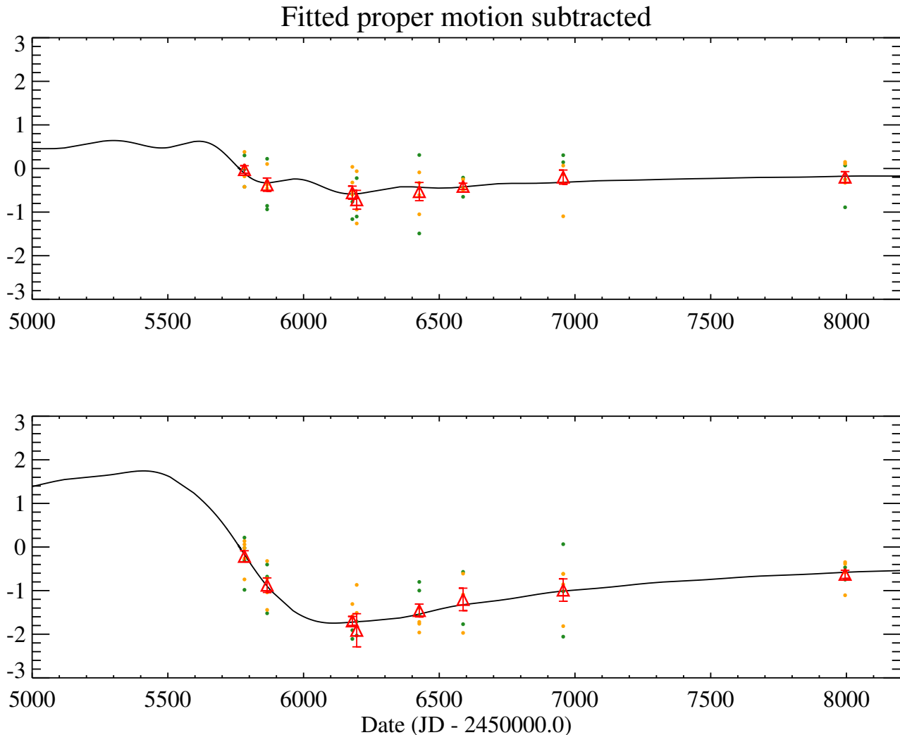
Figure 18. Predicted and measured positions of the source for our adopted joint astrometric and photometric fit. Small dots show the individual measurements from HST images (green for F606W, orange for F814W), while red triangles with error bars show the average and uncertainty at each HST epoch. The black line is our final adopted model. The fitted proper motion for the source has been subtracted from both model and measurements, in order to allow a better scaling of the plot.
