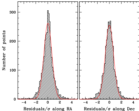
Figure 10. Histogram of the position residuals for all the reference stars in RA and Dec from their proper motion solution, as measured in each image separately, and scaled with the measured dispersion for that star. The scaled residuals closely follow a standard Normal distribution (shown by the red curves). As noted in the caption to Figure 9, reference stars cover a range of magnitudes around the unamplified source magnitude.
