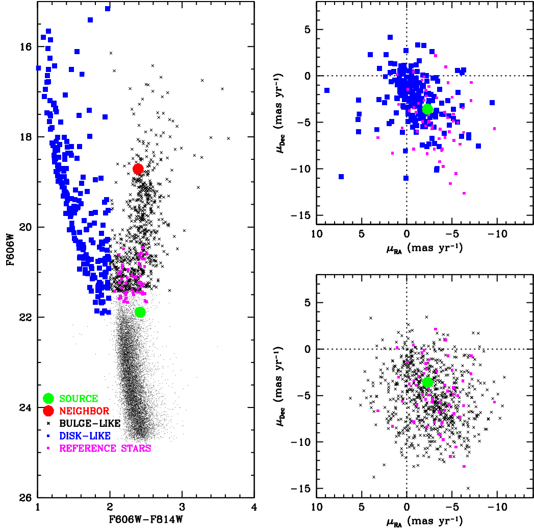
Figure 7. Left panel: color-magnitude diagram [ m_{F606W} versus (m_{F606W} - m_{F814W}) ] for all stars in the HST /WFC3 field. The main-sequence turnoff occurs at m_{F606W} \simeq 22 , above which the disk and the bulge split into two sequences: the redder stars are mainly bulge objects, while the bluer ones are mainly disk objects. Stars marked by blue squares are selected as “disk-like” stars, and the stars marked by black crosses are selected as “bulge-like.” The position of the (unmagnified) microlensed source is shown as a green dot. The nearby bright star 0'.4 away and about 20 times brighter than the unmagnified source is shown as a red dot. Magenta points are the astrometric reference stars used in our analysis. Top right panel: proper motions of the disk-like stars (blue), the reference stars (magenta), and the source (green dot). Bottom right panel: proper motions of the bulge-like stars (black crosses), the reference stars (magenta), and the source (green dot). Only bulge-like stars (shown in magenta) with brightness similar to the observed brightness of the star were used in the final astrometric transformations. This ensures that the reference stars are very similar to the target source star, and uncorrected CTE and small parallax effects should cancel in the differential astrometric measurements.
