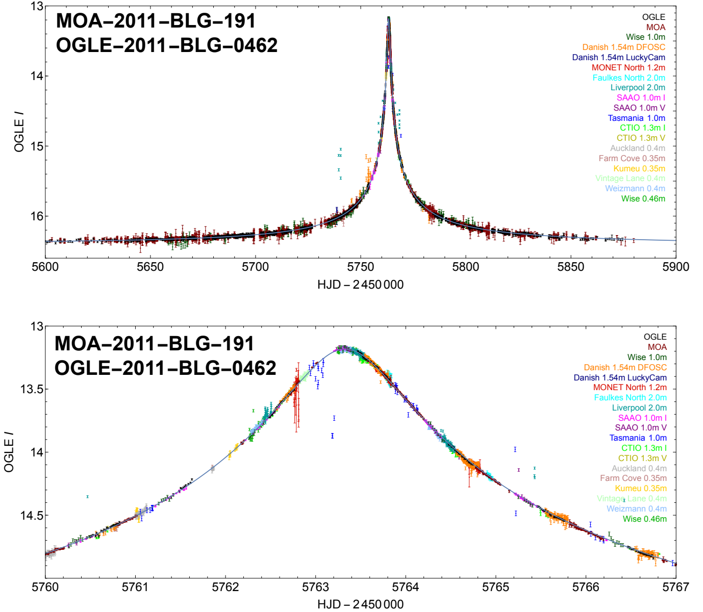
Figure 14. Ground-based photometric observations of MOA-11-191/OGLE-11-462, along with a best-fitting model light curve, shown over a 300-day interval in the upper panel and over a zoomed-in region covering seven days around peak magnification in the bottom panel. All data have been transformed to OGLE I magnitudes according to the inferred baseline magnitudes and blend ratio from the common model.
