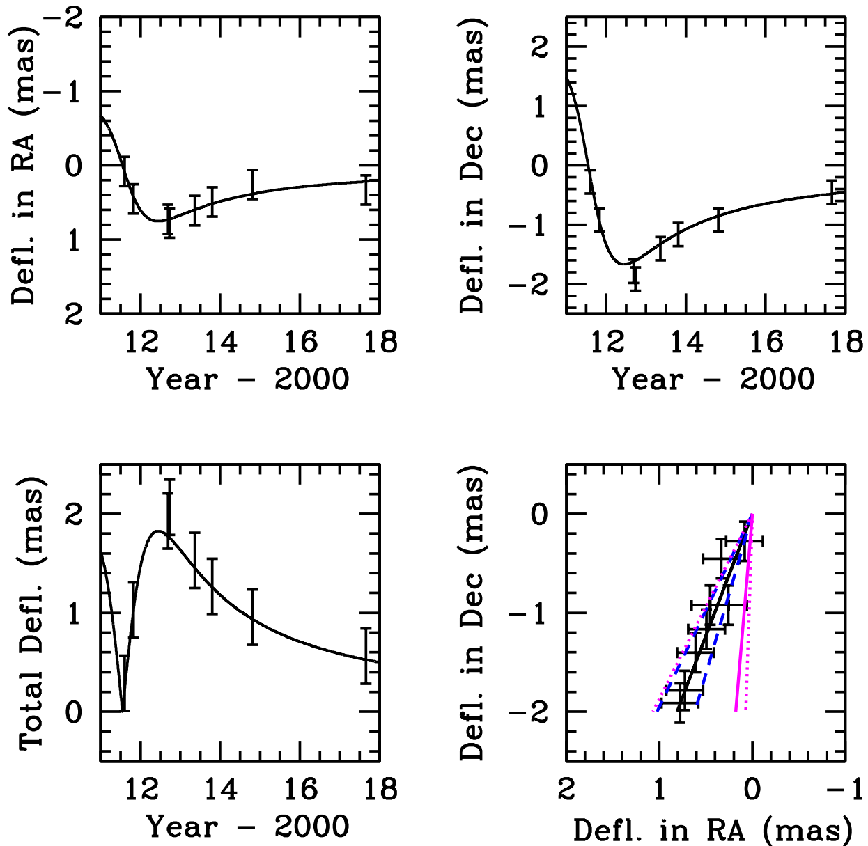
Figure 16. The top two panels show the average values of the measured deflections in RA and Dec at each HST epoch. We use the values of t_0 , t_E , and u_0 as derived from a light-curve fit without parallax, and fit for the proper motion of the source, \theta_E , and \varphi_{LS} . The solid black line is the best fit with \theta_E = 5.2 mas and \varphi_{LS} = 337^\circ.9 . The bottom left panel shows the total deflections at each epoch. The bottom right panel shows the RA versus Dec deflections. These deflections are always along the line joining the lens to the source, and thus at large separations their direction is opposite to the direction of the relative motion of the lens with respect to the source. The solid black line passes through the origin, at the \varphi_{LS} angle derived above. The dotted blue lines indicate the allowed range from astrometry based on the uncertainties. The allowed range of \varphi_{LS} from photometry alone is shown by the dotted magenta lines, the best fit value being \varphi_{LS} = 354^\circ.8 shown by the solid magenta line. The combined constraint from photometry and astrometry is used in our subsequent analysis.
