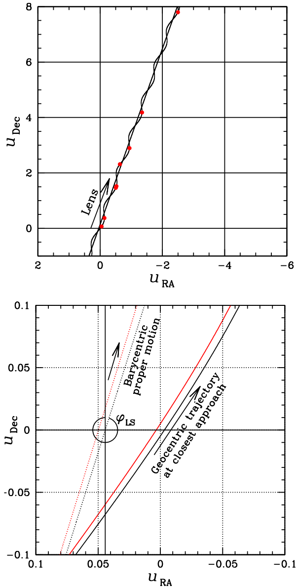
Figure 15. Top panel: path of the lens with respect to the source, the position of the source being fixed at (0,0). The direction of motion is shown by an arrow. The black straight line is the lens path without parallax, and the wavy line is the path including parallax. Red points mark the epochs of HST observations. u_{RA} and u_{Dec} are the RA and Dec components of the lens-source separation, in units of \theta_E . Bottom panel: enlarged view of the lens trajectory with respect to the source around closest angular approach. Black lines correspond to the u_{0,-} solution, which is the preferred solution, and the red lines show the less-preferred u_{0,+} solution. In both cases, the barycentric trajectories (no parallax), shown by dotted lines, pass on the north side of the source. The geocentric trajectory (i.e., the trajectory as seen by an observer on Earth, which includes parallax) of the u_{0,+} solution (shown by the solid red line) passes on the north side of the source, but the trajectory of the u_{0,-} solution (shown by the black solid line) passes to the south. The u_{0,-} solution is used in our analysis presented here. It is worth noting, however, that the derived \theta_E , and hence the mass of the lens, is nearly identical for both solutions. \varphi_{LS} is the position angle of the barycentric proper motion of the lens with respect to the source (i.e., no parallax), as shown here.
