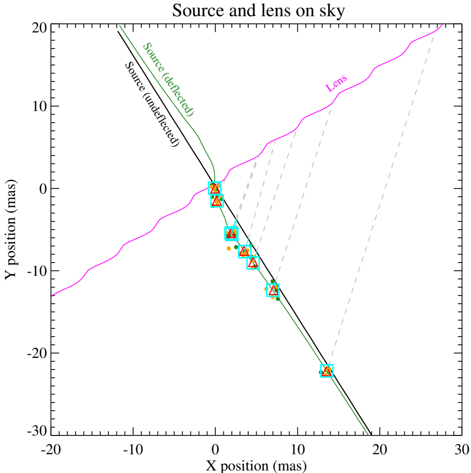
Figure 17. Representation of the reconstructed motions of the lens and of the source on the plane of the sky. The reference point is the undeflected position of the source at time t_0 . The small dots are the individual measurements from HST images (green for F606W, orange for F814W); the larger red triangles represent the average positions for each epoch. The cyan squares are the fitted positions at each epoch. The gray lines connect the undeflected source and lens positions at each HST epoch.
