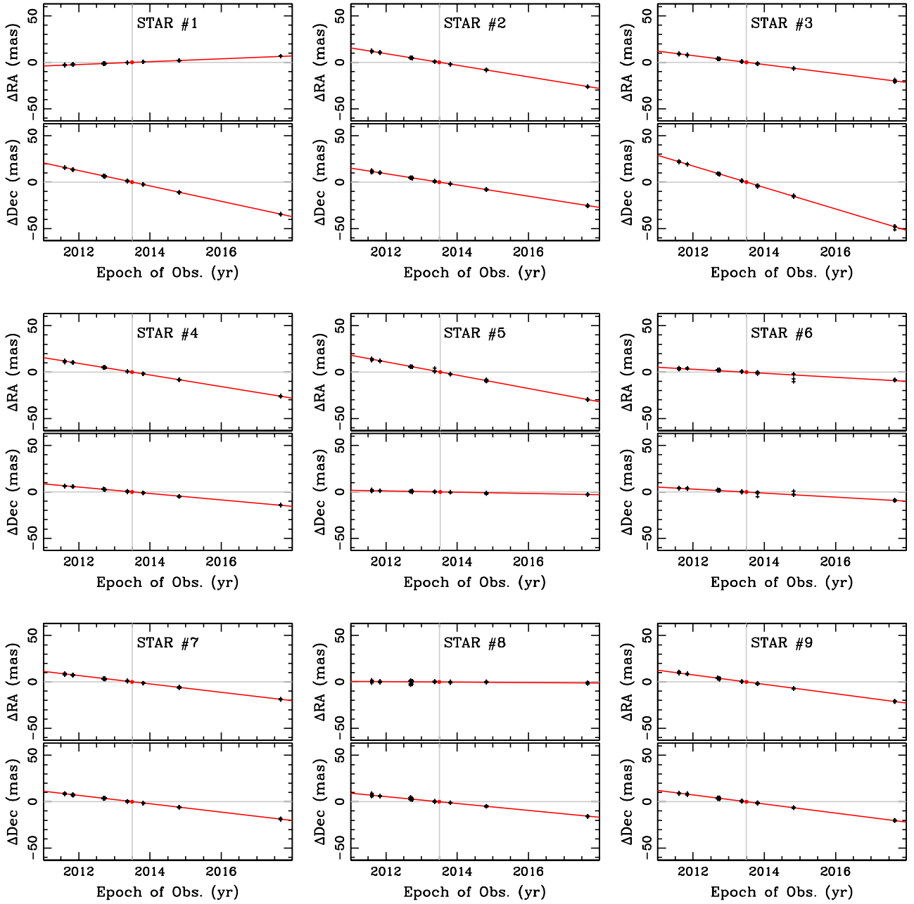
Figure 8. Motions of nine representative astrometric reference stars in right ascension and declination. The red lines are linear fits to the proper motions of the stars.
