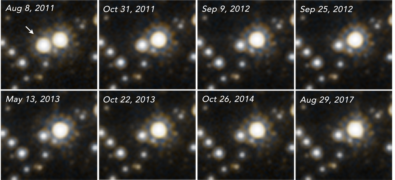
Figure 5. 2''.1 \times 2''.0 cutouts around MOA-11-191/OGLE-11-462 as observed by HST at all 8 epochs. Exposures were taken in F606W and F814W from 2011 to 2017; see Table 2 for details. The source star is marked by an arrow in the first-epoch (top left) image. At this epoch, on 2011 August 8, the magnification was a factor of \sim 12 . The maximum astrometric deflection occurred at Epochs 3 and 4, when the photometric magnification was only about 10%. In 2017, the source had returned very close to its unmagnified brightness and undeflected position.
