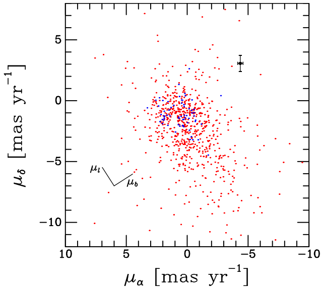
Figure 22. Proper-motion components from Gaia EDR3 for a sample of stars at similar distances to that of the black hole, selected as described in the text. Typical uncertainties are about \pm 0.05 \text{ mas yr}^{-1} in both coordinates. Blue points represent a younger main-sequence population with Gaia colors of G_{\text{BP}} - G_{\text{RP}} < 1.0 , and red points an older and dynamically hotter population. The directions of Galactic longitude and latitude are indicated at the lower left. The black point with error bars shows the proper motion of the black hole, which is a significant outlier compared to the surrounding population.
