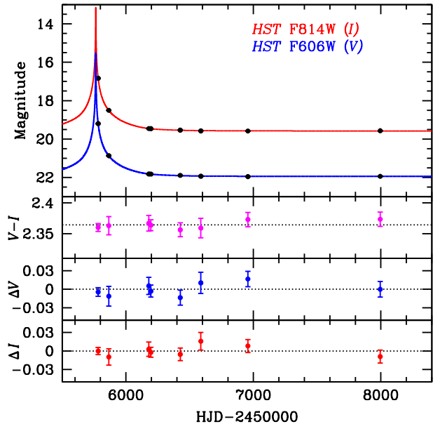
Figure 13. Top panel: Photometry of MOA-11-191/OGLE-11-462, obtained with HST over 6 years at 8 epochs in the F606W ( V ) and F814W ( I ) filters (black filled circles), along with our final model fits from §8.2 (red and blue curves). Errors on the photometry are smaller than the plotting points. The second panel plots the observed values of V - I , showing that the source color remained constant to within \sim 0.01 mag during the entire 6-year duration. The third and fourth panels show that the residuals, V_{\text{obs}} - V_{\text{model}} and I_{\text{obs}} - I_{\text{model}} , at the epochs of the HST observations are consistent with zero within the measurement uncertainties (see §8.2 for more details and discussion).
