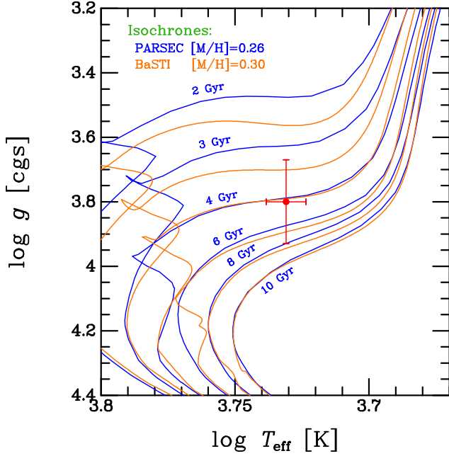
Figure 19. Location of the MOA-11-191/OGLE-11-462 source star in the \log g versus effective-temperature diagram (red filled circle with error bars), using stellar parameters from Bensby et al. (2013). Superposed are theoretical isochrones from two sources. The blue curves show PARSEC isochrones, calculated for the source’s measured metallicity of [M/H] = +0.26 , for ages of 2 to 10 Gyr. The orange curves are BaSTI isochrones for [M/H] = +0.3 and the same range of ages.
