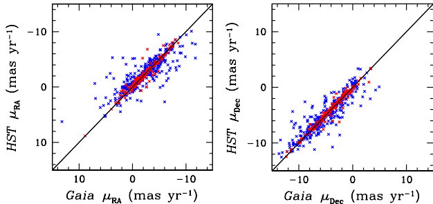
Figure 6. Proper motions of the reference stars used in our analysis derived from our HST observations with a 6-year baseline, versus the Gaia proper motions. Red points represent stars brighter than G = 18 , for which the Gaia errors are typically < 0.2 \text{ mas yr}^{-1} , and blue points represent fainter stars for which the errors are larger. Our analysis uses the Gaia reference frame, so it is natural that there is good agreement between them. But the individual HST measurements have higher precision, particularly at fainter magnitudes.
