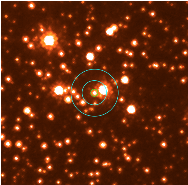
Figure 4. HST image in the F814W ( I -band) filter of an 8'' \times 8'' region centered on MOA-11-191/OGLE-11-462, obtained at our final epoch in 2017 August. North is at the top, east on the left. Encircled in green is the source star, now returned to baseline luminosity. The site is resolved into the source, a much brighter neighboring star 0''.4 to the WNW, and several nearby fainter stars. The inner cyan circle has a diameter of 1'' , corresponding to the typical best seeing in ground-based microlensing survey images; the outer cyan circle’s diameter is 2'' , which is not unusual seeing. The source, bright neighbor, and several fainter stars are generally blended in ground-based frames, and the blending increases with seeing.
