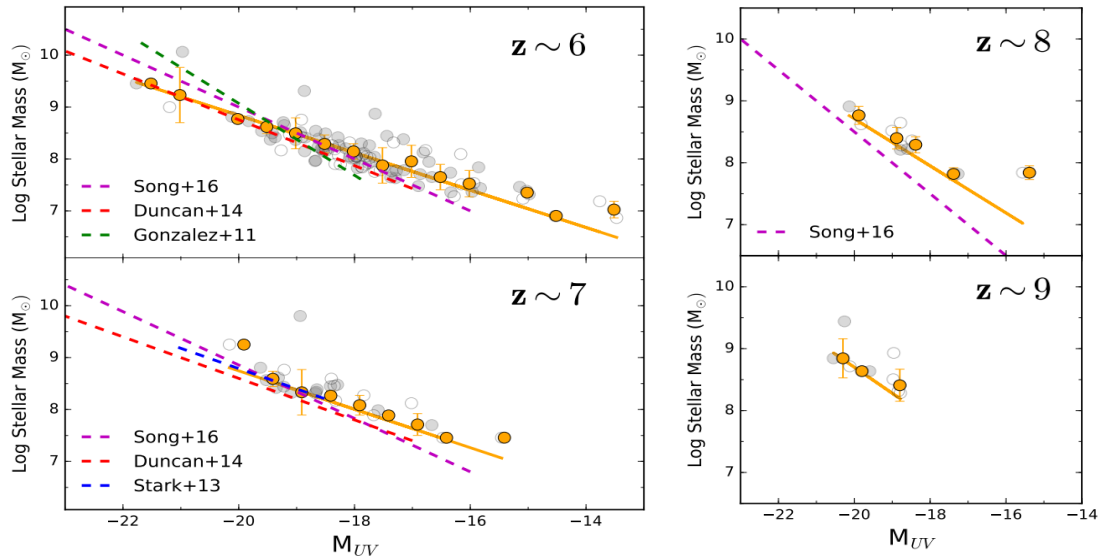
Figure 15. Stellar mass as a function of rest-frame absolute UV magnitude at 1500 angstrom at z = 6 - 9 . Grey filled circles represent sources with a S/N ratio > 3\sigma at 3.6\mu\text{m} in IRAC, whereas grey open circles are those with a S/N ratio \lesssim 3\sigma . Filled yellow circles represent the median stellar masses in each rest-frame absolute UV magnitude bin of 0.5 mag, and the yellow error bars represent the standard deviation in stellar mass in each UV magnitude bin. The best-fit \log_{10}(M_*/M_\odot) - M_{UV} relation is shown by solid yellow line in each redshift bin. The best-fit \log_{10}(M_*/M_\odot) - M_{UV} lines of González et al. (2011), Stark et al. (2013), Duncan et al. (2014) and Song et al. (2016) are also shown by green, blue, red and magenta dashed lines, respectively, for comparison.
