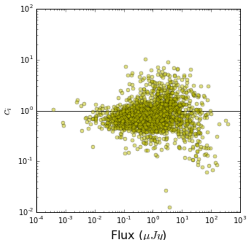
Figure 5. Covariance index c_i as a function of measured fluxes from T-PHOT for the MACS0416 cluster. 527 (16 per cent) sources from our catalog lie above c_i > 1 and are treated with caution.
