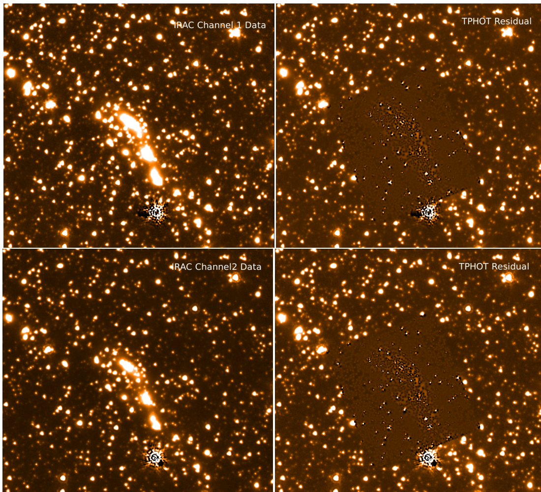
Figure 4. IRAC 3.4\ \mu\text{m} and 4.5\ \mu\text{m} imaging of the MACS0416 cluster. Top left: Example of severely blended sources in IRAC channel 1 low resolution image. Top right: Residual image from T-PHOT. Bottom left: Original IRAC channel 2 image. Bottom right: Residual image from T-PHOT.
