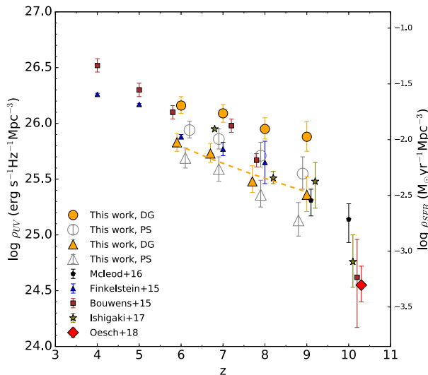
Figure 18. Evolution of UV luminosity density as a function of redshift. \rho_{UV} values calculated with a M_{UV} = -13.5 limit are shown in orange filled circles and \rho_{UV} calculated using a M_{UV} = -17 limit are shown in orange filled triangles. Also shown are the \rho_{UV} estimates considering point sources in our completeness simulations with open grey circles and open grey triangles for M_{UV} = -13.5 and M_{UV} = -17 respectively. The literature points shown are estimated with a M_{UV} = -17 limit. The dashed yellow line is the power-law fit to the data points at z \sim 6-9 , such that \rho_{UV} \propto (1+z)^{-2.63} . Fitting a power-law at z \geq 8 values results in \rho_{UV} \propto (1+z)^{-4.61} (not shown).
