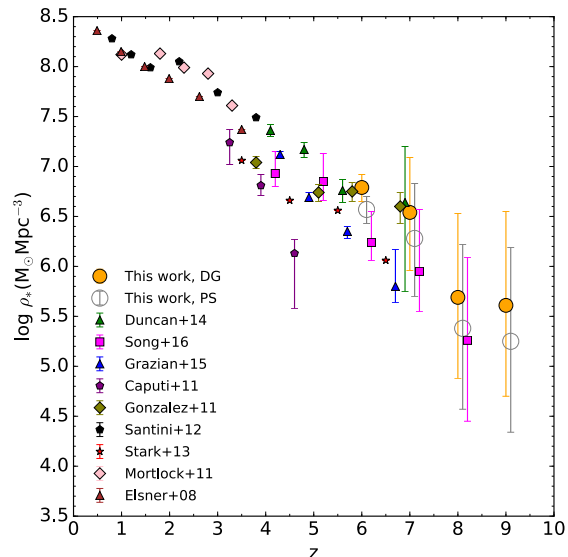
Figure 16. Evolution of total SMD as a function of redshift. We calculate the total SMD by integrating the best fit Schechter function from M_* = 10^8 to 10^{13} M_\odot for our GSMFs. The quoted 1\sigma error bars represent the minimum and maximum range of stellar mass densities within the 1\sigma contours of Schechter parameters obtained from our MCMC analysis. Our results are shown as solid orange points when disc-like galaxies are considered in our completeness simulations, and as open grey circles considering point sources. Shown also are the values from the literature converted to a Chabrier IMF, where necessary.
