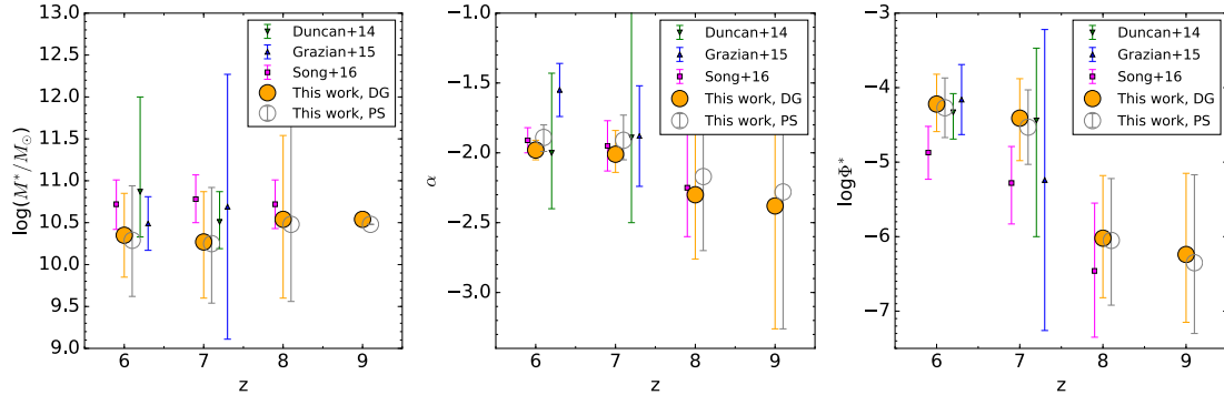
Figure 14. Redshift evolution of best fit Schechter function parameters for our stellar mass functions. The solid orange circles represent the best fit Schechter parameters considering disc-like galaxies in our completeness simulations, whereas the open circles are our results considering point sources. The low mass end slope \alpha steepens with increasing redshift, number density \Phi^* decreases with increasing redshift, whereas no evolution in the characteristic mass M^* is observed. Note: The error bars on characteristic mass M^* at z \sim 9 are not shown since we keep the value of M^* fix to the value estimated at z \sim 8 .
