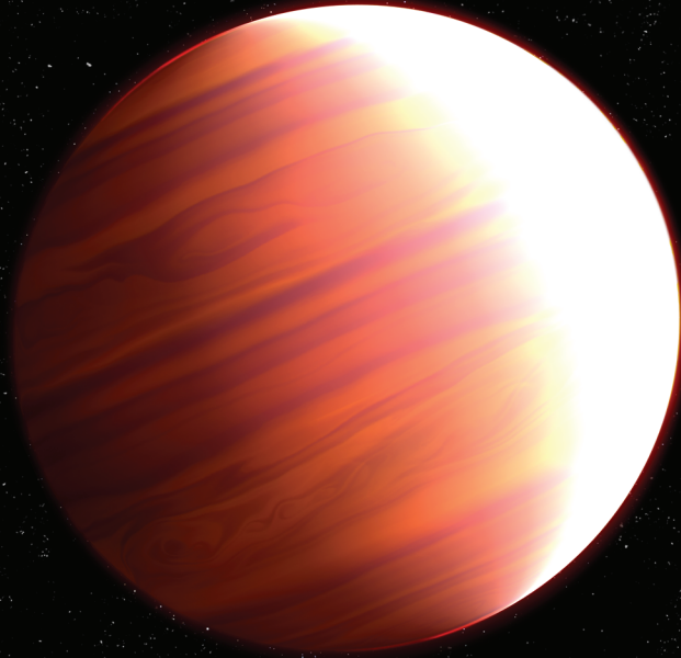
Kepler-13Ab
