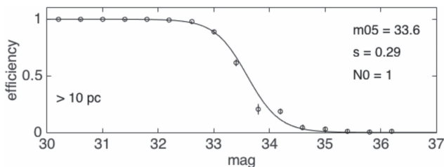
Figure 12. Model fits to the empirical efficiency for clumps larger than 10 pc, as a function of clump magnitude. The best-fit parameters to Equation (8) for each size bin are shown in the upper right-hand corner.
