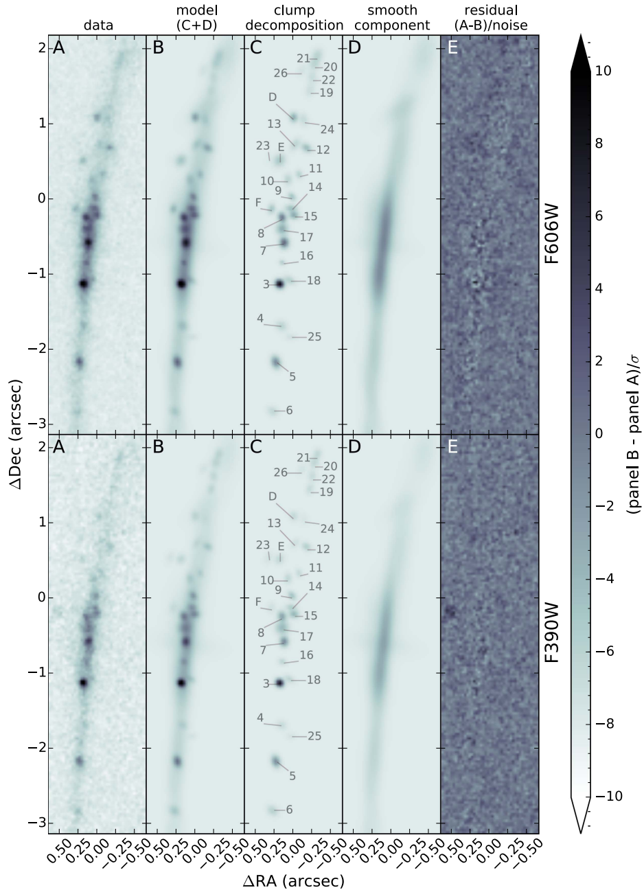
Figure 9. GALFIT clump decomposition in F606W (top) and F390W (bottom) imaging. (A) HST imaging of the middle image of SGAS J111020.0+645950.8 in the image plane. (B) The complete GALFIT model of the middle image of the arc. (C) Clump component of panel B. (D) Smooth component of panel B. (E) Residual of the clump+smooth GALFIT model and the data in units of rms noise.
