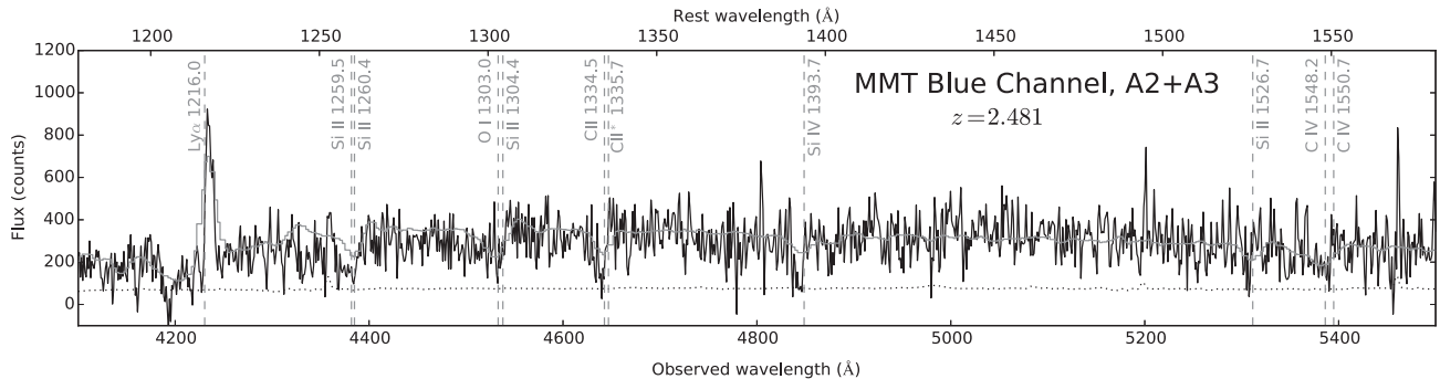
Figure 4. MMT Blue Channel Spectrograph spectrum of SGAS J111020.0+645950.8. The dotted line indicates the noise level, and the gray-solid line is a spectral template of Ly \alpha -emitting galaxies with strong absorption features at z \sim 3 galaxies from Shapley et al. (2003). The vertical gray-dashed lines indicate the locations of rest-frame UV emission and absorption lines.
