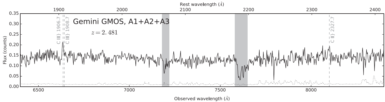
Figure 2. Gemini GMOS spectrum of SGAS J111020.0+645950.8, summed from slits placed on all three images (A1, A2, and A3). The dotted line indicates the noise level, and the gray bands indicate part of the spectrum with strong telluric absorption. The vertical gray-dashed lines indicate the locations of rest-frame UV emission lines.
