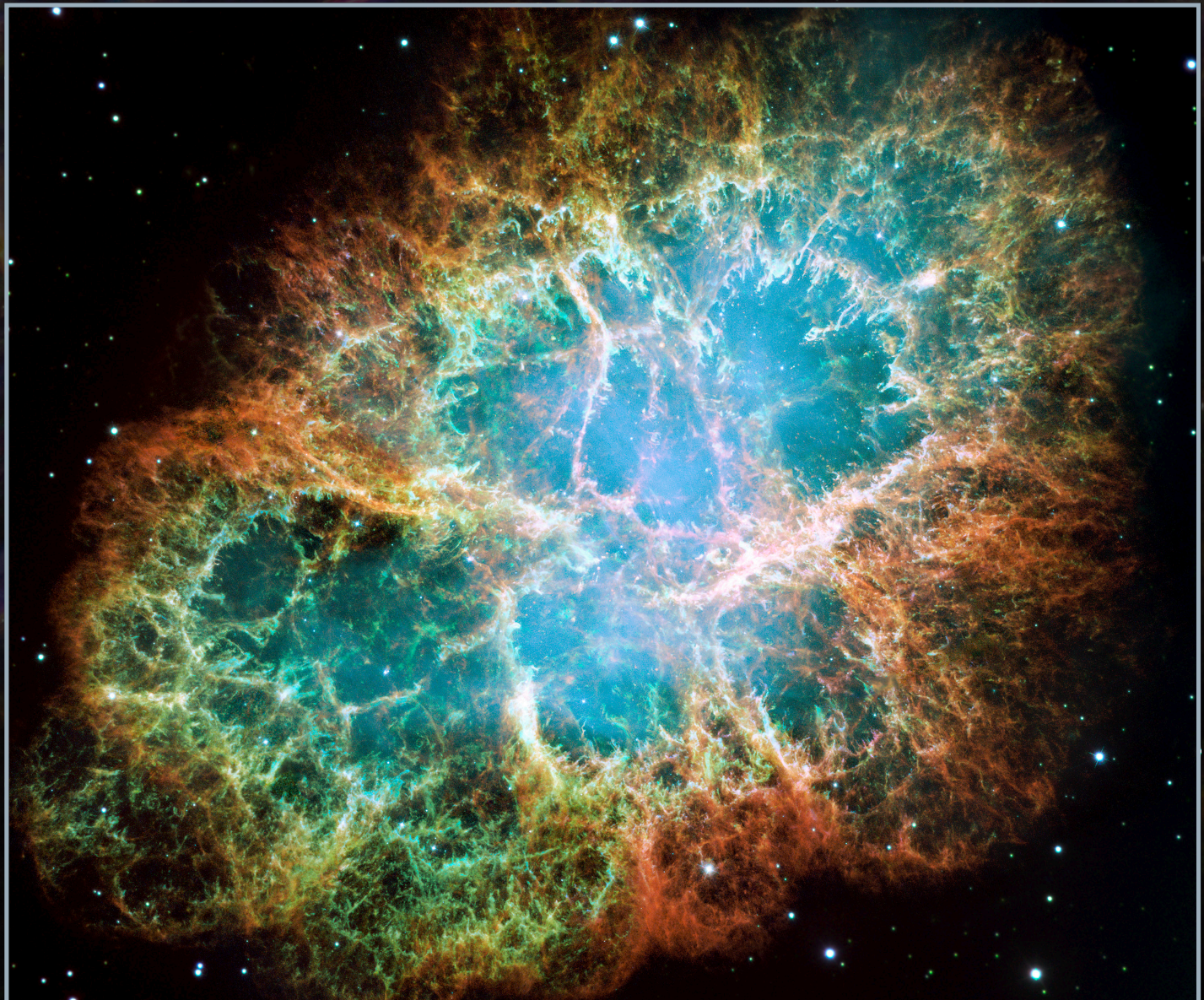
M1, the Crab Nebula, is the remnant of a stellar explosion that was seen in Earth's skies in the year 1054 AD. The colors in the image were assigned to distinguish various chemical elements, which are now all racing into space to enrich new generations of stars.
