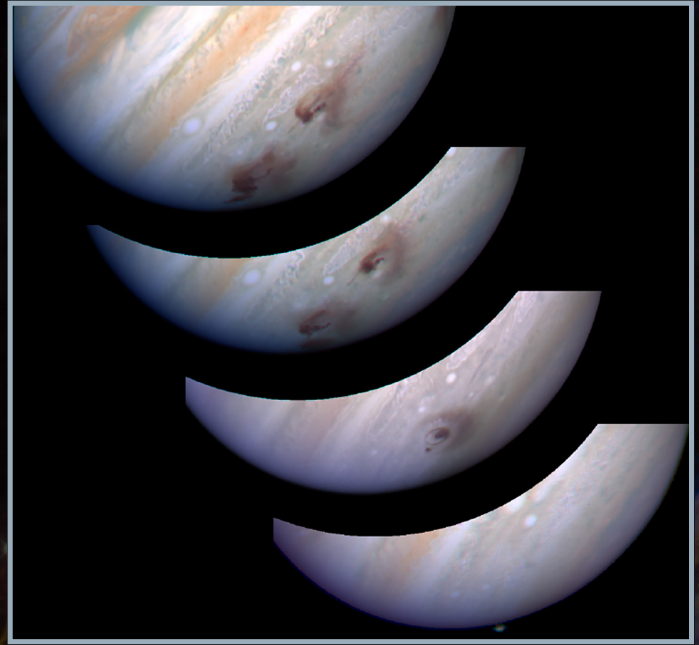
This image series, starting in the lower right corner, shows the darkening of Jupiter's clouds as a result of the impact of Comet Shoemaker-Levy 9.
