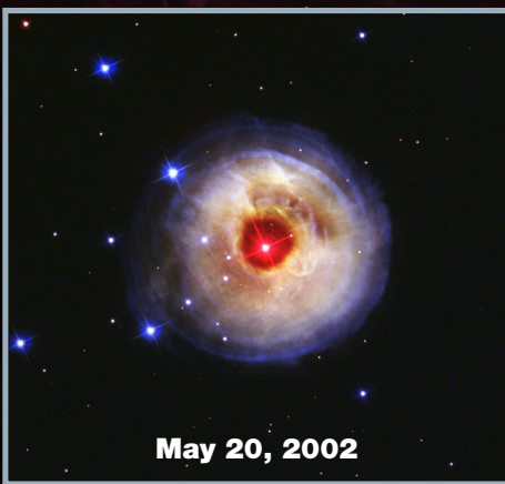
A mysterious flash from the red giant star V838 Mon illuminated the surrounding area in a light echo.
