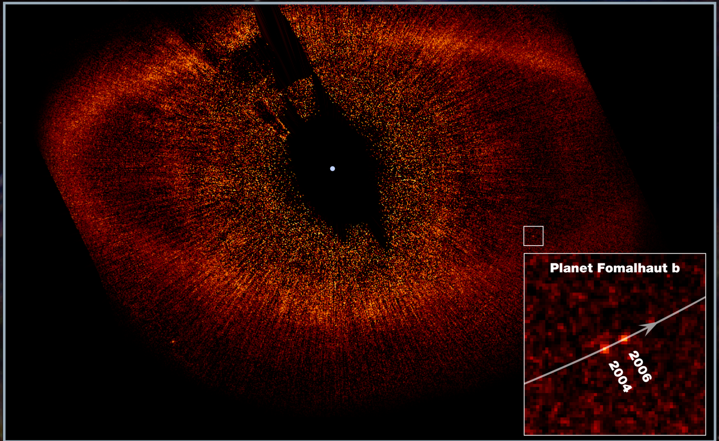
Astronomers used Hubble to take one of the first-ever visible-light pictures of an extrasolar planet, named Fomalhaut b .
