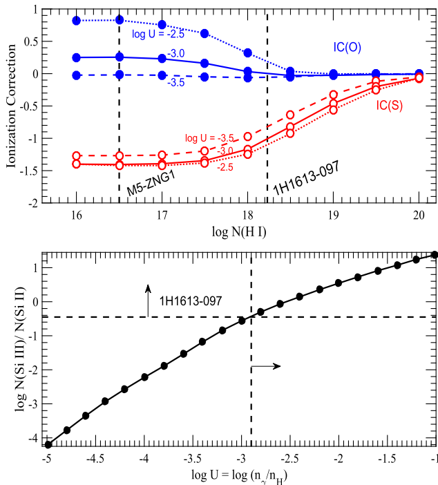
Figure 4. Upper panel: Ionization corrections IC(O) and IC(S) against H I column density for a uniform-density photoionized cloud. The values of N(H I) appropriate for the HVCs toward 1H1613-097 and M5-ZNG1 are shown with dashed vertical lines. These corrections are used to convert [O I/H I] into [O/H] . Lower panel: Dependence of the ion ratio N(Si III)/N(Si II) on \log U for the case of the HVC at -172 \text{ km s}^{-1} toward 1H1613-097. The measured value of the ratio is used to constrain \log U , which in turn is used to constrain IC(O) .
