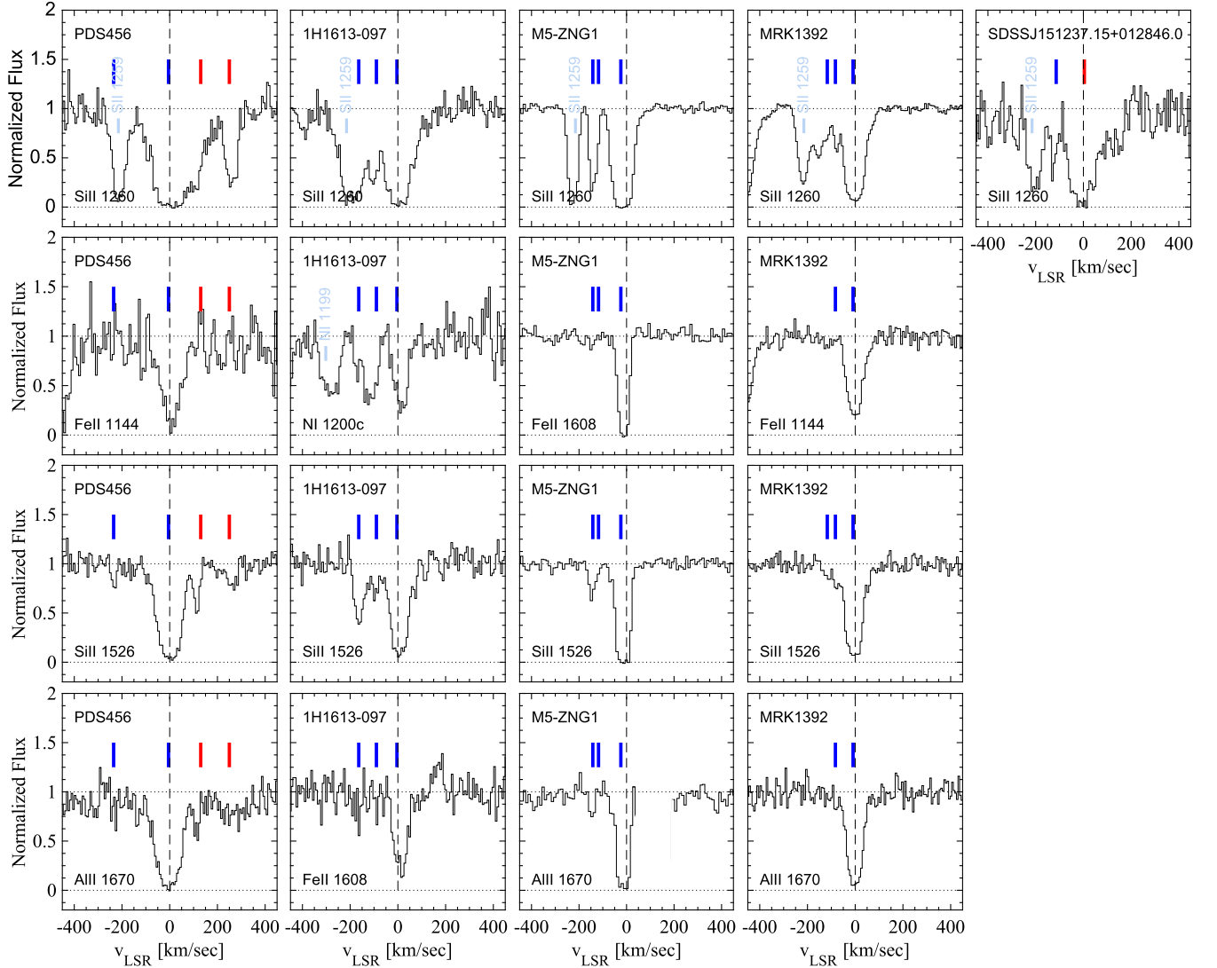
Figure 9. HST -COS spectra of additional transitions for the five lines of sight inside the northern Fermi Bubble. The vertical ticks indicate the velocities of HVCs along these directions. Both the redshifted components (red ticks) and blueshifted components (blue ticks) are flagged.
