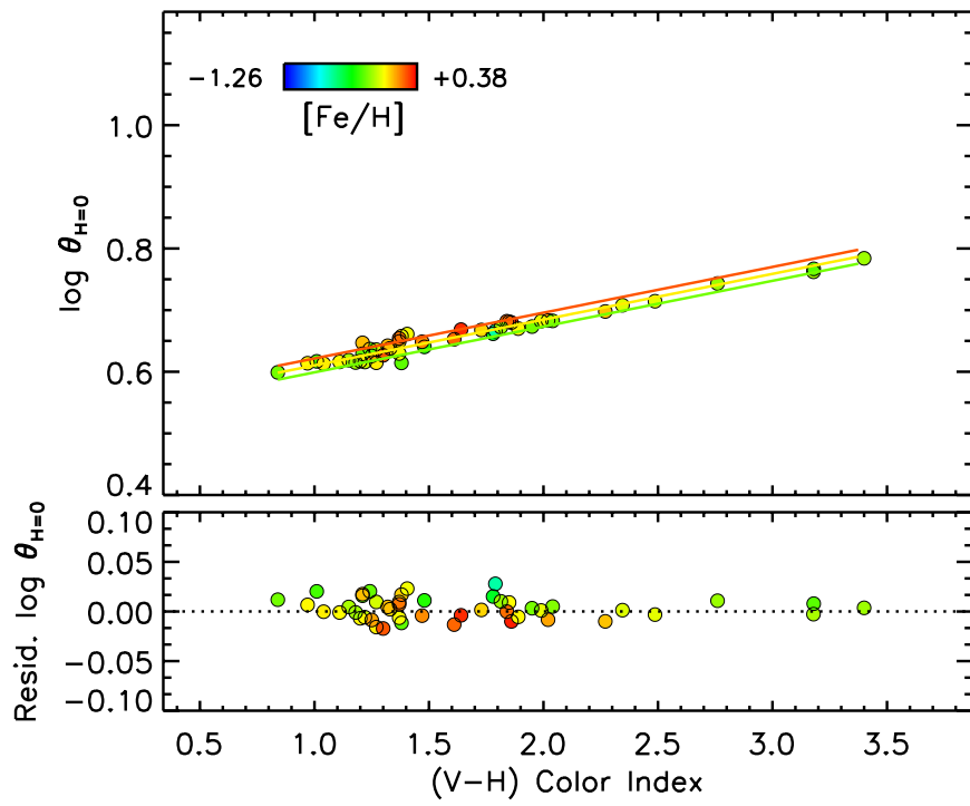
Fig. 7.— The V - H , H angular source size relation from the analysis of Boyajian et al. (2014), including the effect of metallicity.
