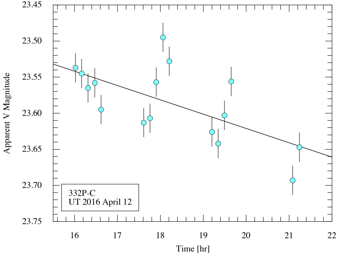
Fig. 4.— Photometric variations in 332P-C measured on UT 2016 April 12. Error bars of \pm 0.02 magnitudes are shown. The solid line is a linear fit to the data to show secular fading at 0.016 magnitudes per hour.
