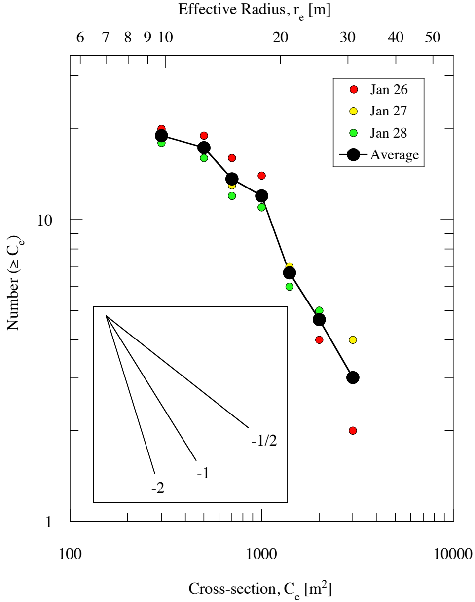
Fig. 3.— Cumulative distribution of fragment cross-sections, C_e , computed from Equation (2), (lower axis, in m 2 ) and effective radii given by r_e = (C_e/\pi)^{1/2} (upper axis, in m). Large black circles show the average counts from UT 2016 January 26, 27 and 28 while small colored circles show the individual counts. The inset shows gradients 1 - g = -1/2, -1 and -2 , for reference.
