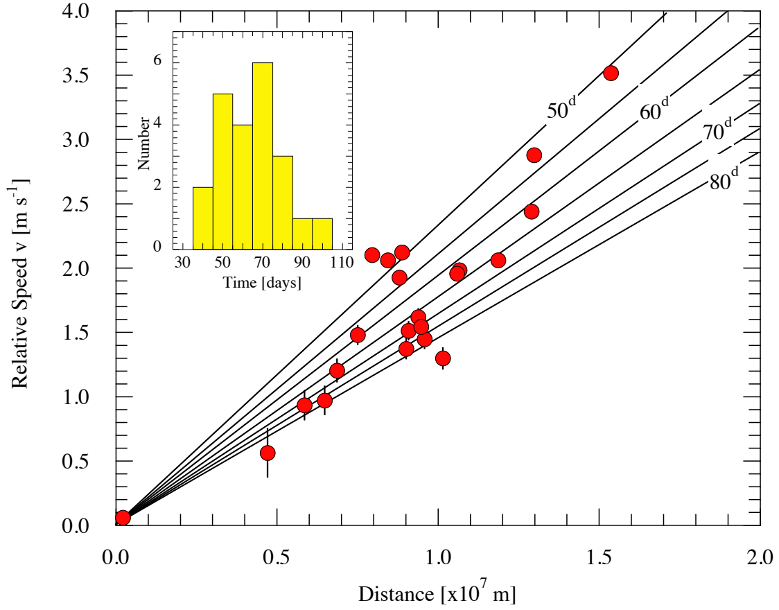
Fig. 2.— Measured fragment velocities as a function of sky-plane distance, both with respect to parent body “C”. Diagonal lines show different times since ejection, labeled in days. The inset plots the distribution of travel times.
