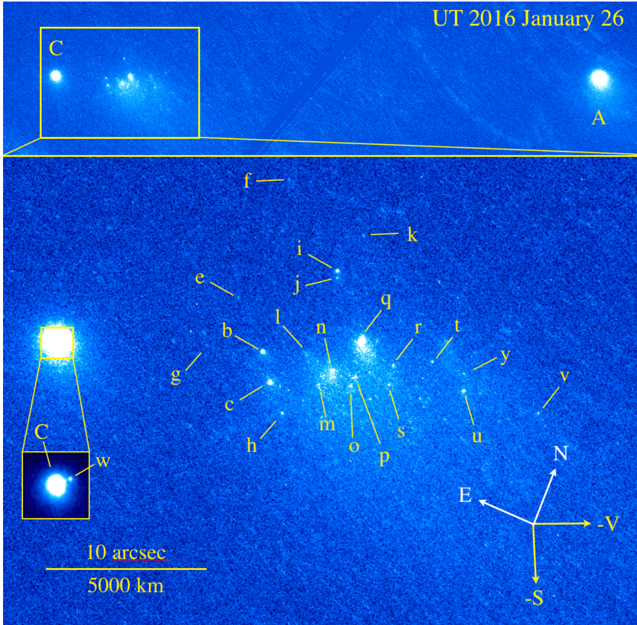
Fig. 1.— 332P on UT 2016 January 26 showing fragments measured in this work. The image has been rotated to bring the axis of the object to the horizontal. The wide panel at the top identifies the bright objects A and C (the parent nucleus). A yellow box marks the region shown in the main panel, with measured fragments identified. A further 2'' wide zoom box is included to reveal fragment w in the glare of C . Arrows show the cardinal directions and the projected negative velocity vector, -V , and the antisolar direction, -S , from Table (1).
