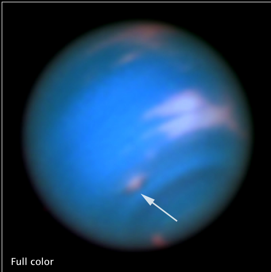
Dark Spot on Neptune ■ May 16, 2016 Hubble Space Telescope ■ WFC3/UVIS
