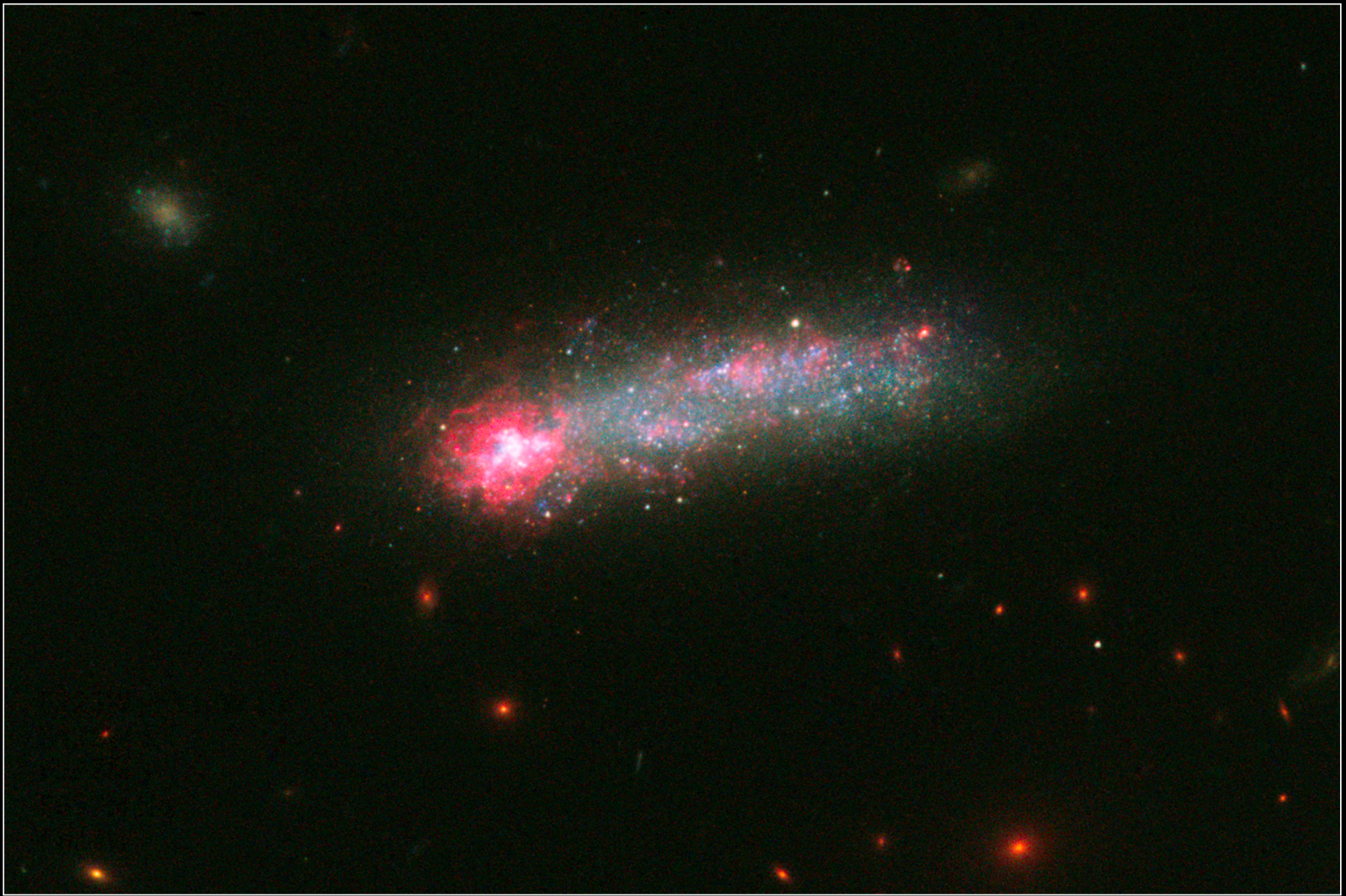
Dwarf Galaxy Kiso 5639 Hubble Space Telescope • WFC3/UVIS
