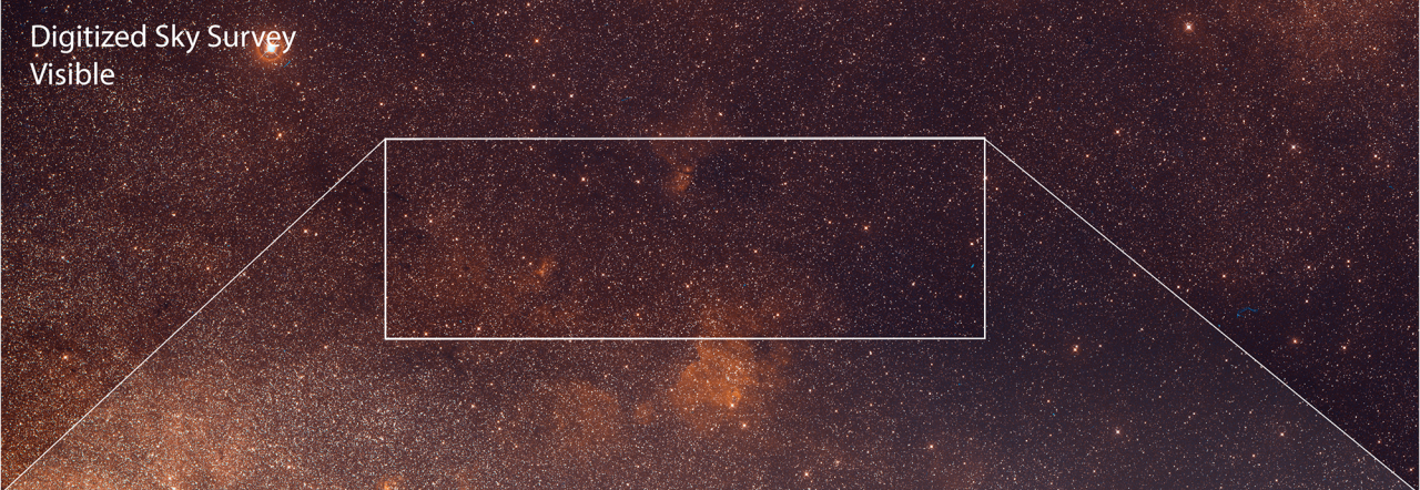
Spitzer Space Telescope Infrared
