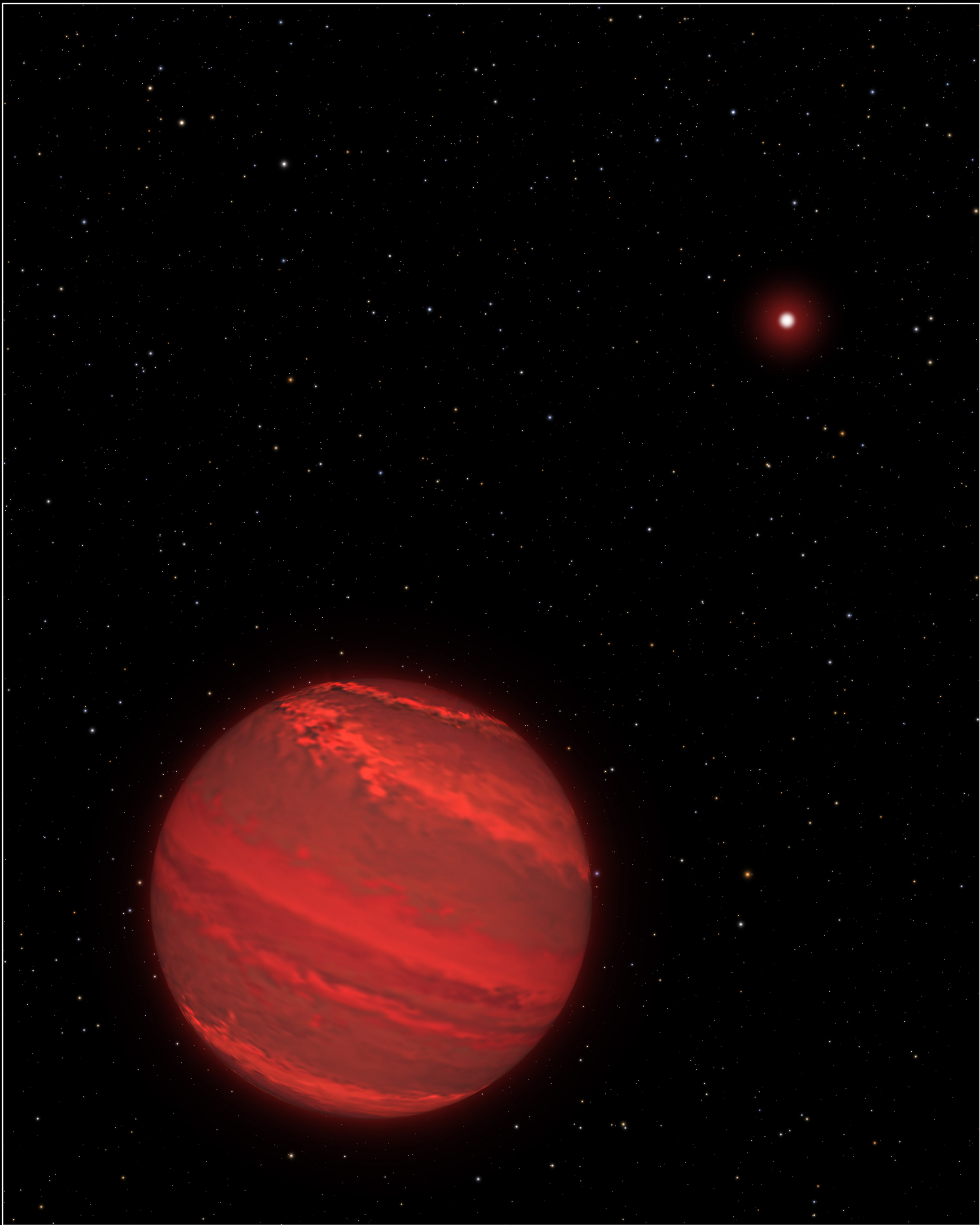
Artist's View of a Super-Jupiter around a Brown Dwarf (2M1207)
