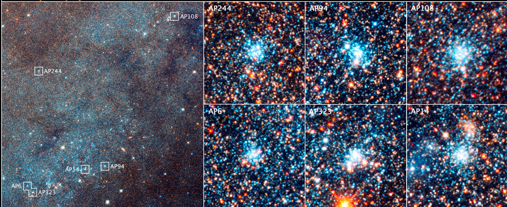
Star Clusters in the Andromeda Galaxy HST ■ WFC3/UVIS/IR ■ ACS/WFC
