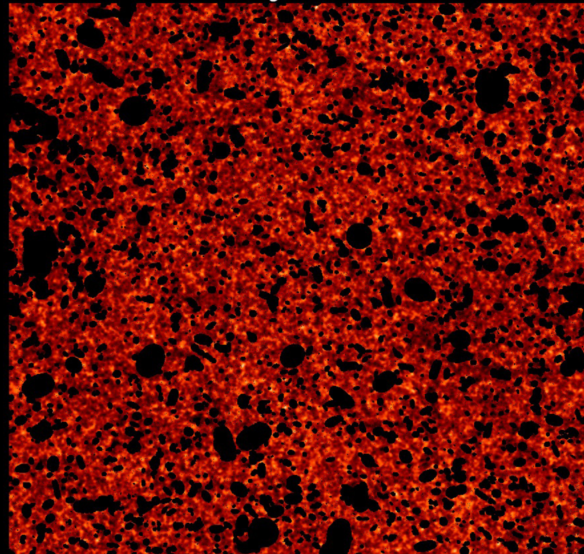
First Light Galaxies
