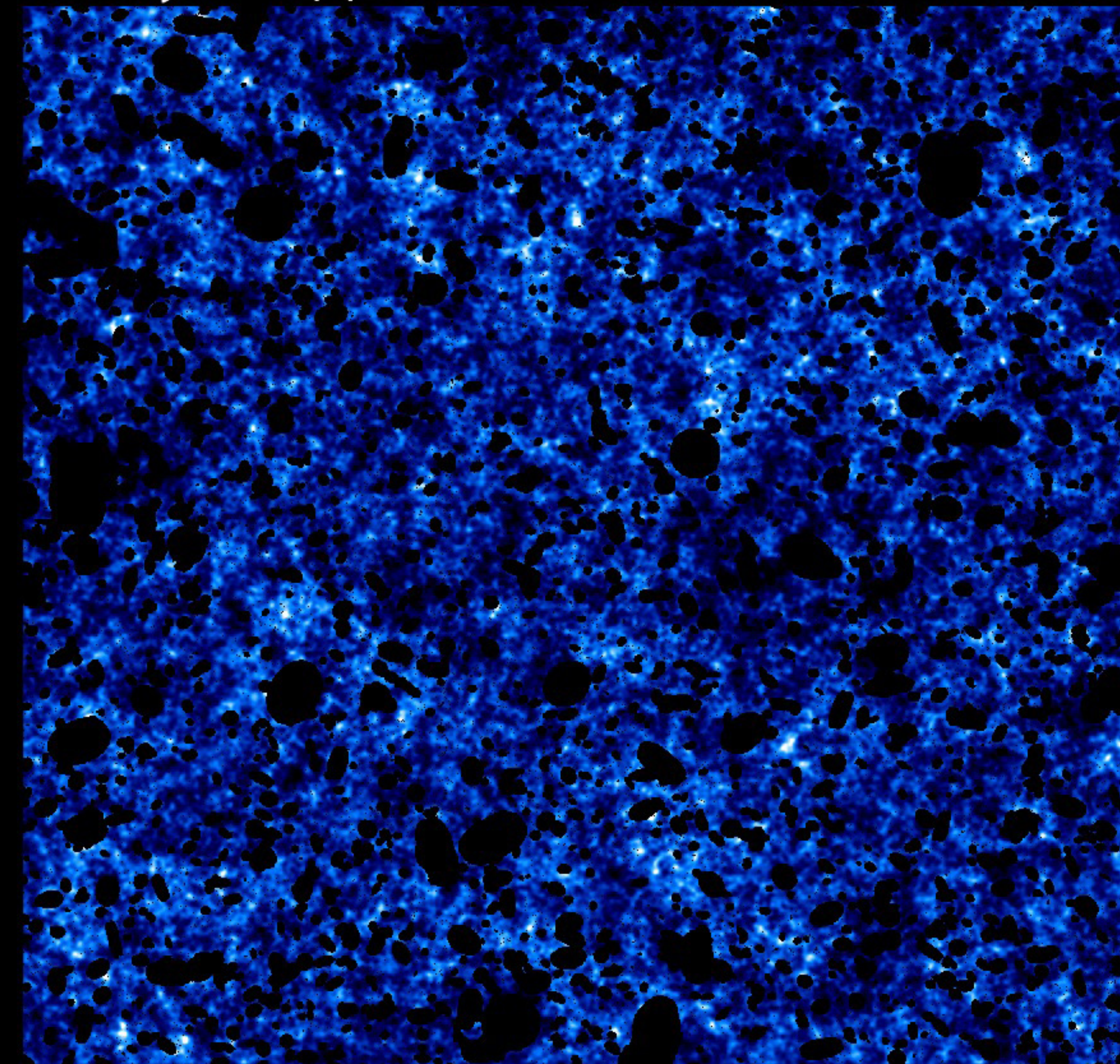
Tidally Stripped Stars between Galaxies
