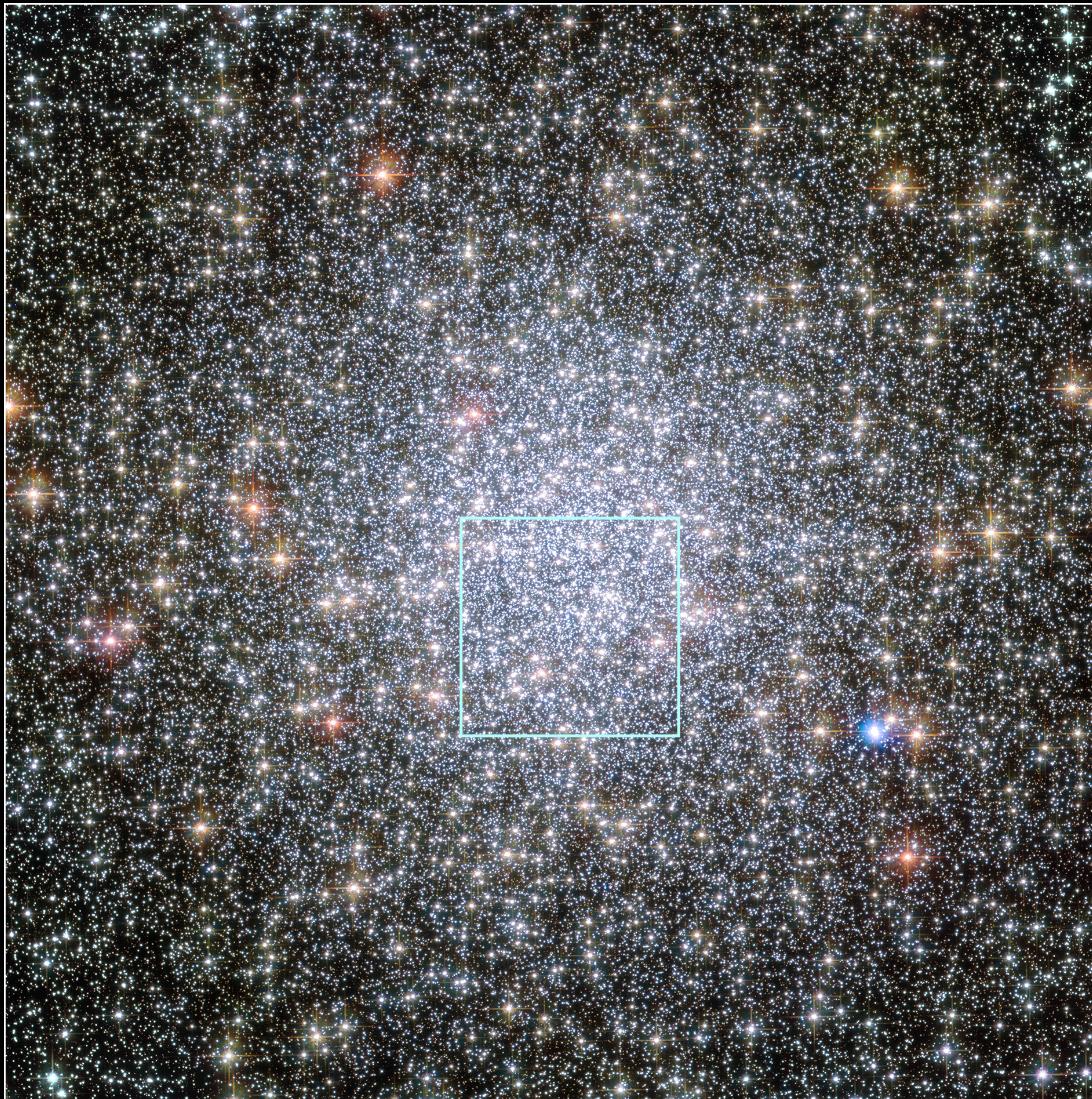
Globular Cluster 47 Tucanae Hubble Space Telescope ■ ACS/WFC ■ WFC3/UVIS
