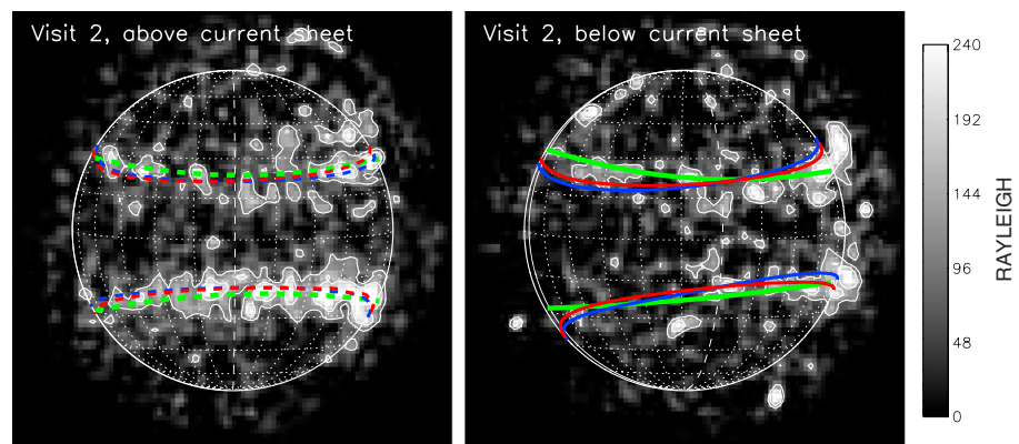
Figure 4. Visit 2: Observed auroral brightness in Rayleigh at OI 1356 Å when Ganymede is (left) above and (right) below the current sheet. Other properties are similar as in Figure 3.
