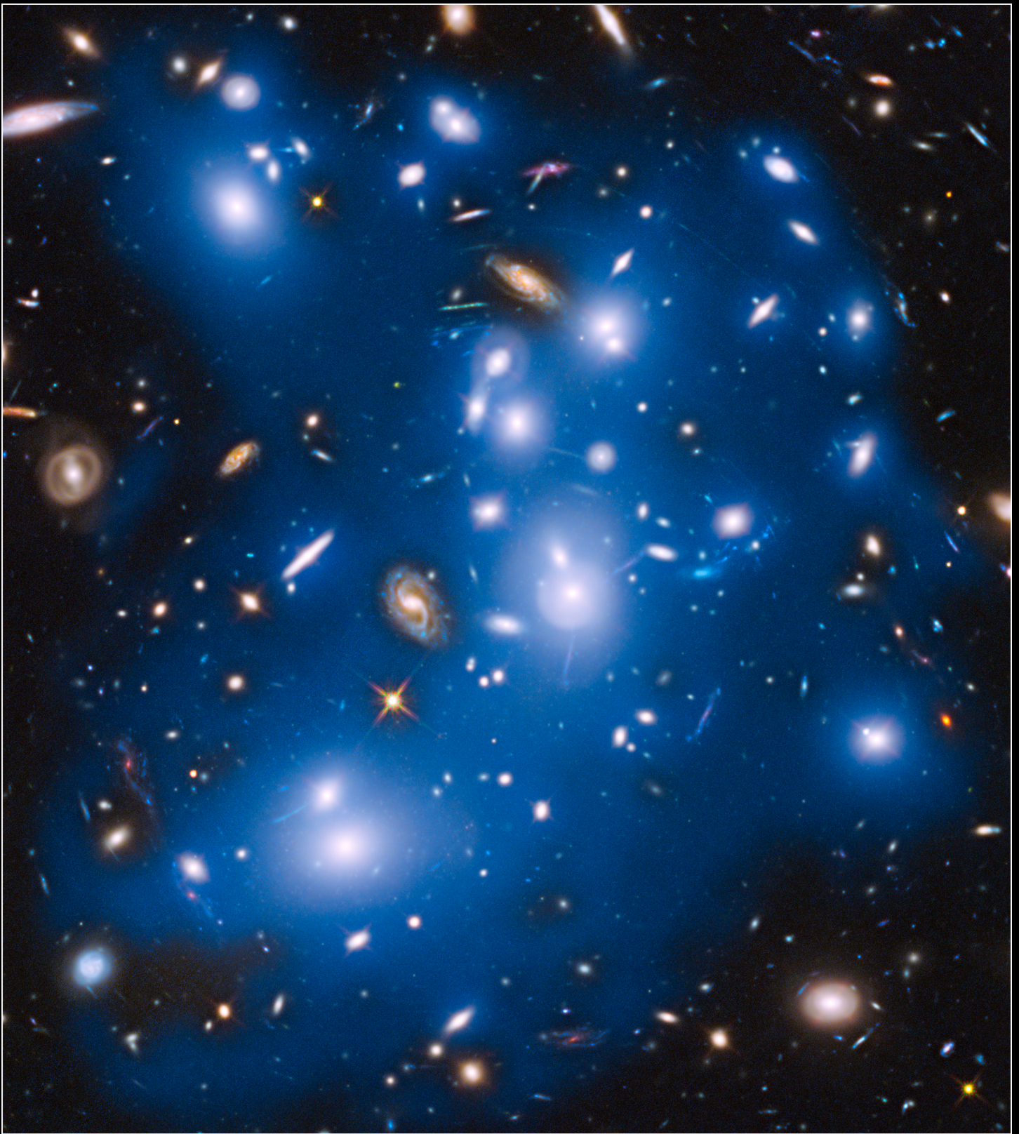
“Ghost Light” in Galaxy Cluster Abell 2744 Hubble Space Telescope • ACS • WFC3
