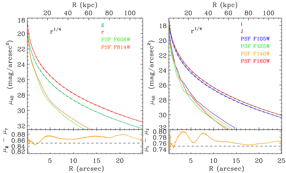
Figure 3. Upper panels: surface brightness profiles of the models (dashed lines) and the convolved models (solid lines) for the ACS (left hand panel) and WFC3 (right hand panel) filters used in the analysis. The PSF profiles in all the observed used bands are also shown. The bottom panels show the effect of the PSF in the restframe colors: g - r (left) and i - J (right). The input model colors are indicated with dashed lines.
