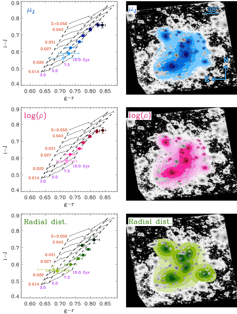
Figure 1. Left panels show the i - J vs. g - r diagrams for three different parameters: \mu_J (blue), \log(\rho) (pink), and R (green) used to characterize the different spatial regions where the light of the cluster is distributed. Overplotted is a color grid prediction based on Bruzual & Charlot (2003) models using a Salpeter IMF for single stellar populations. Right panels show the image of the cluster in the F160W filter and overplotted are the different spatial regions in which the colors are measured. The spatial regions are coded from the inner parts of the cluster (darker color) to the outer parts (lighter color).
