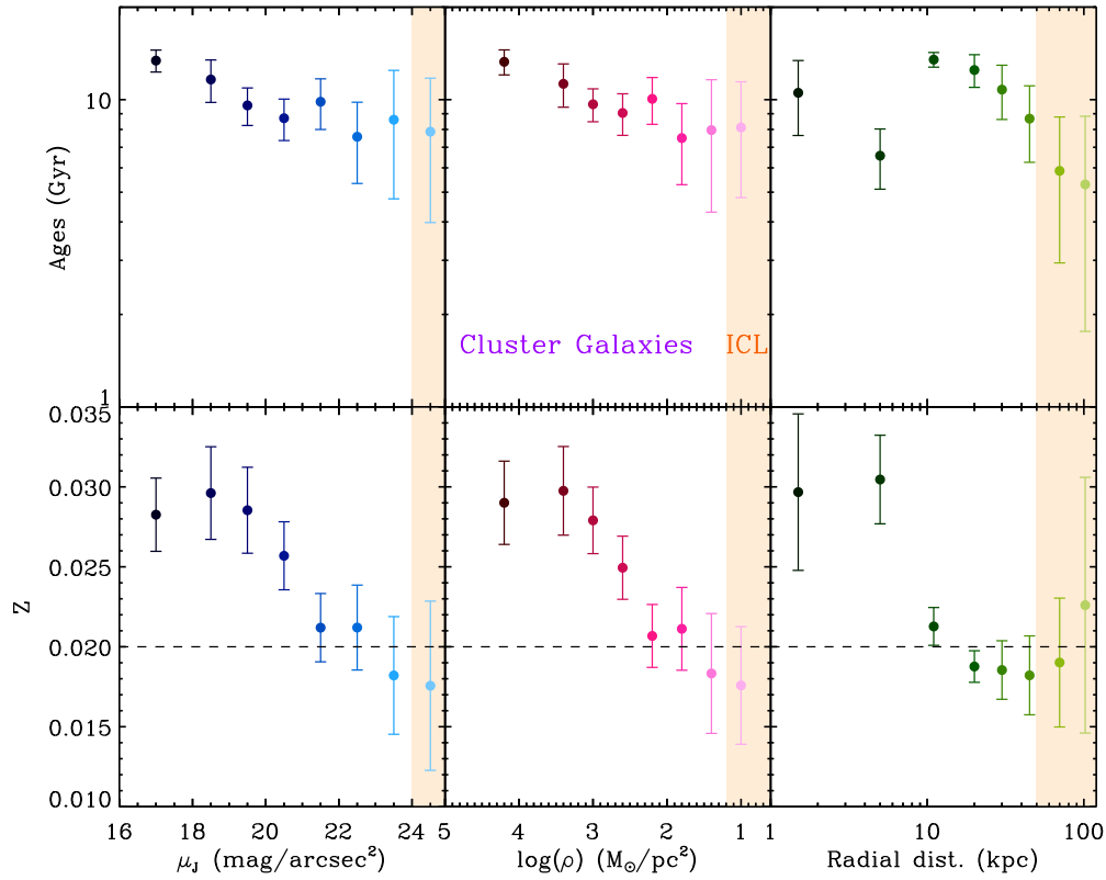
Figure 2. Gradients of age and metallicity as a function of \mu_J , \log(\rho) , and R . The regions corresponding to the cluster galaxies (purple) and the ICL (orange) are labeled. The dashed line indicates the solar metallicity.
