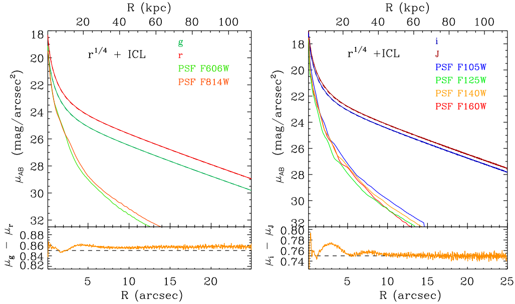
Figure 4. Same as in Figure 3, but adding an ICL component of scale length 18 kpc and \mu_J = 24.5 mag arcsec ^{-2} at R = 50 kpc. (A color version of this figure is available in the online journal.)
