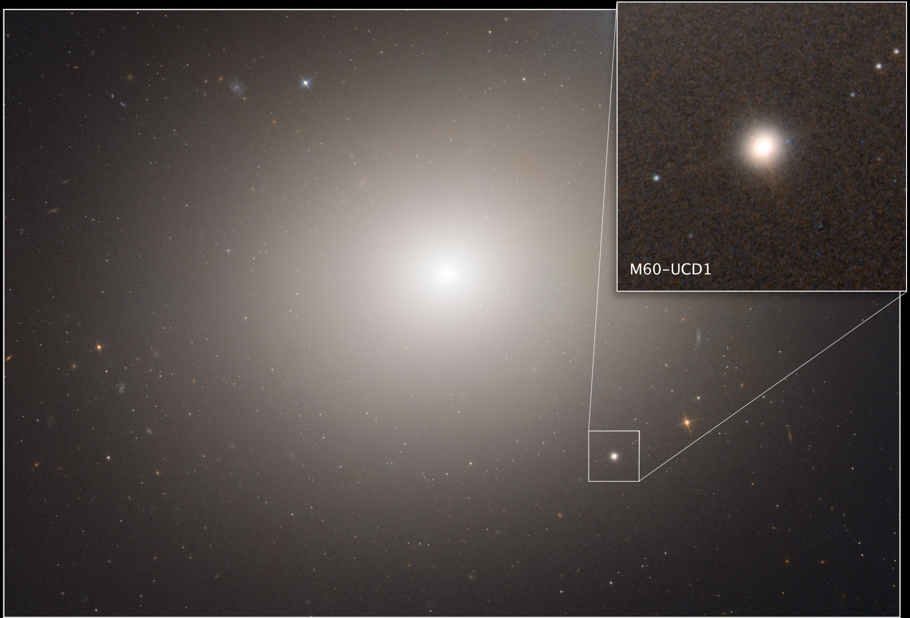
Ultracompact Dwarf Galaxy near Elliptical Galaxy M60 Hubble Space Telescope ■ ACS ■ WFPC2
