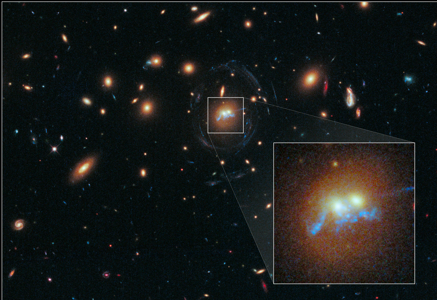
Galaxy Cluster SDSS J1531+3414 Hubble Space Telescope ■ WFC3
