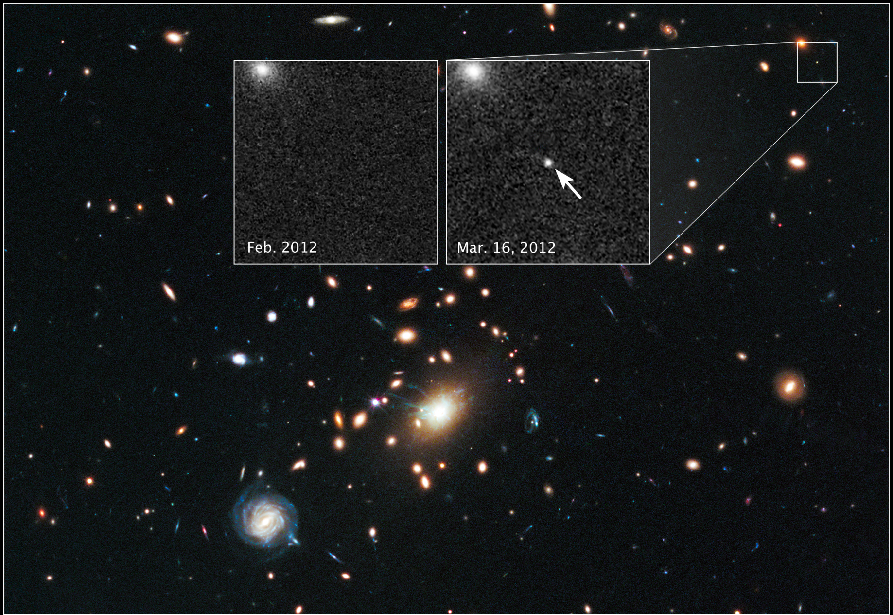
Galaxy Cluster RXJ1532.9+3021 ■ Supernova Didius Hubble Space Telescope ■ ACS/WFC WFC3/IR
