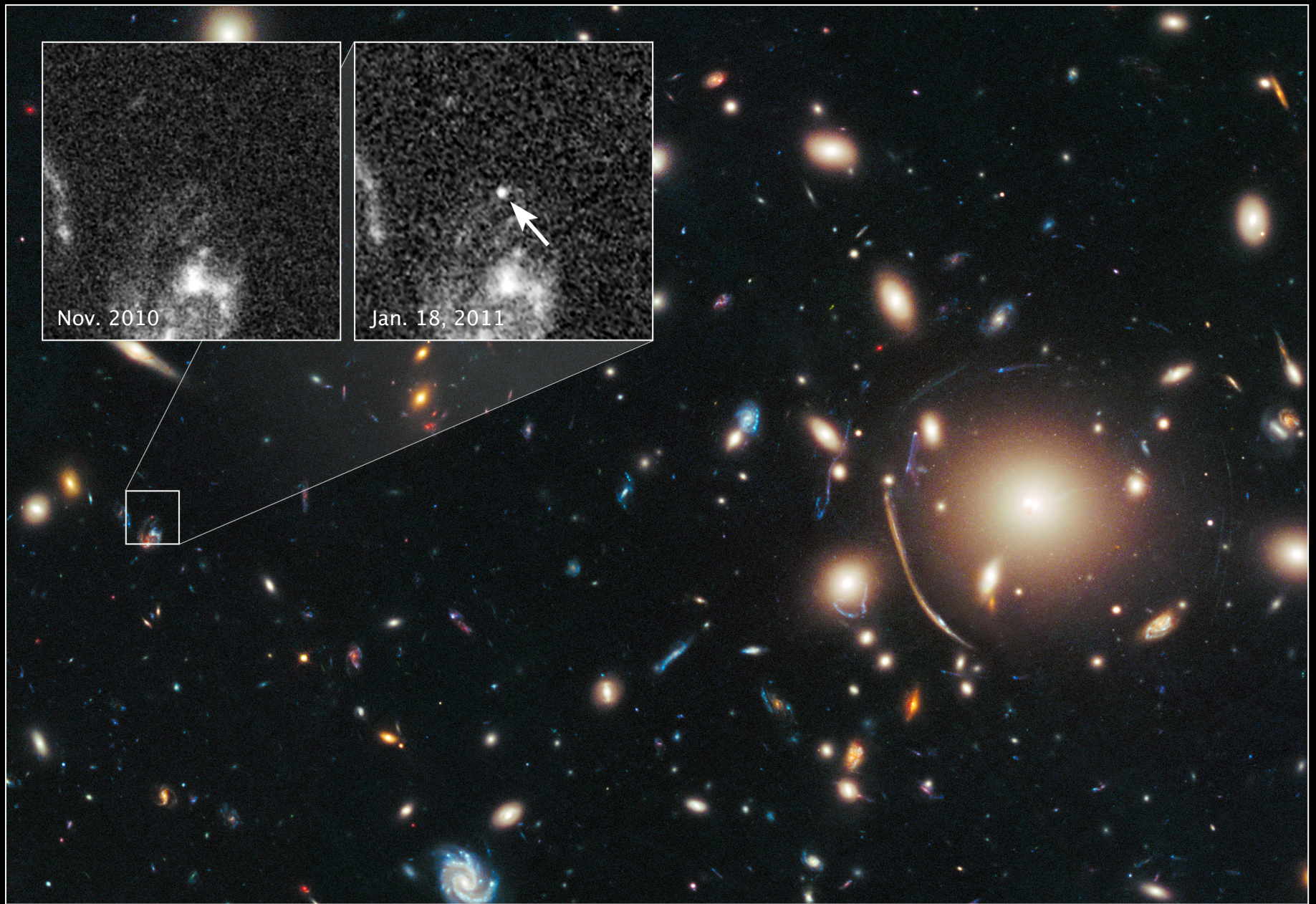
Abell 383 ■ Supernova Tiberius Hubble Space Telescope ■ ACS/WFC WFC3/IR
