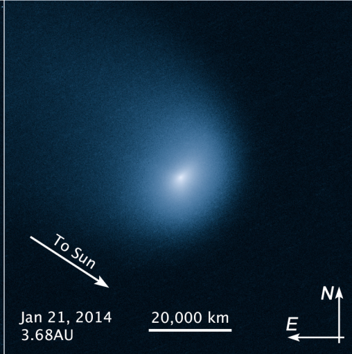
Comet C/2013 A1 (Siding Spring) HST WFC3/UVIS F606W
