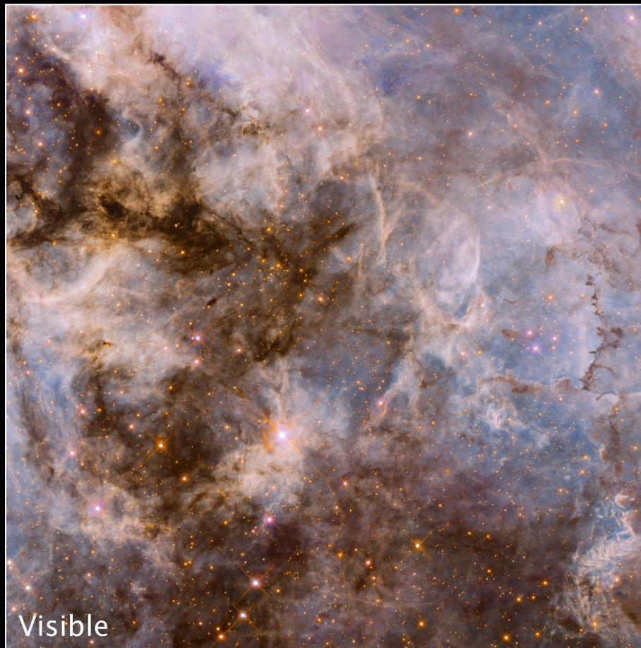
30 Doradus Details Hubble Space Telescope • ACS/WFC • WFC3/IR
