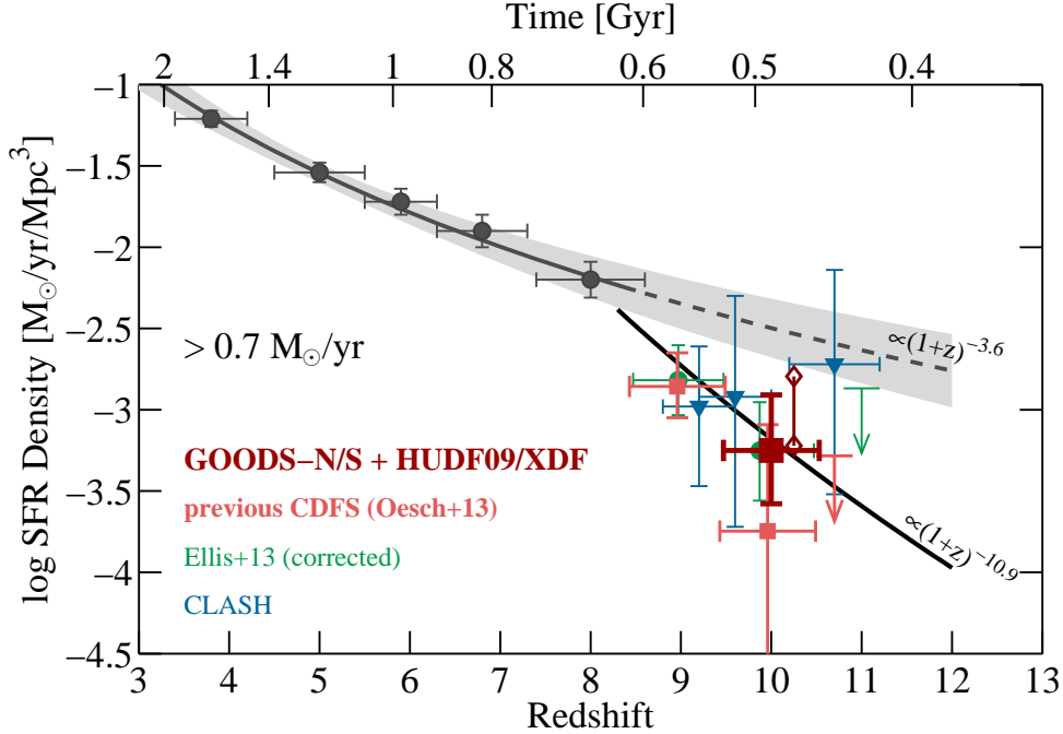
FIG. 9.— The redshift evolution of the cosmic star-formation rate density (SFRD) \dot{\rho}_* above a star-formation limit > 0.7 M_{\odot} \text{yr}^{-1} including the new GOODS-N z \sim 10 galaxy candidates. The lower redshift SFRD estimates are based on LBG UV LFs from Bouwens et al. (2007, 2012b) including dust corrections. The gray band represents their 1\sigma uncertainty. The new measurement from the five detected candidates in the combined CANDELS GOODS-N/S and the HUDF09/12/XDF dataset is shown as the dark red square. The individual SFRD with errorbars were computed from the UV LD of the individually detected sources. Open diamonds connected with a vertical line represent the SFRDs as estimated based on integrating the best-fit UV LFs down to the corresponding luminosity limit of M_{UV} = -17.7 (see Table 4). The upper diamond represents M_* evolution, and the lower diamond is derived from \phi_* evolution. These estimates are offset to z = 10.25 for clarity. Previous measurements of the SFRD at z > 8 are shown from a combination of HUDF09/12+GOODS-S (pale red; Oesch et al. 2013b) as well as from CLASH cluster detections (blue triangles; Bouwens et al. 2012a; Coe et al. 2013; Zheng et al. 2012). Additionally, we also show the results of the HUDF12 field only from Ellis et al. (2013) (green circles). We corrected down their z \sim 10 point by a factor 2\times to account for our removal of a source that was shown to be a diffraction spike (see Oesch et al. 2013b). When combining all the measurements of the SFRD at z \geq 8 from different fields we find \log \dot{\rho}_* \propto (1+z)^{-10.9 \pm 2.5} (black solid line), significantly steeper than the lower redshift trends which only fall off as (1+z)^{-3.6} (gray line). The current data at z > 8 show that the cosmic SFRD is very likely to be increasing dramatically, by roughly an order of magnitude, in the 170 Myr from z \sim 10 to z \sim 8 .
