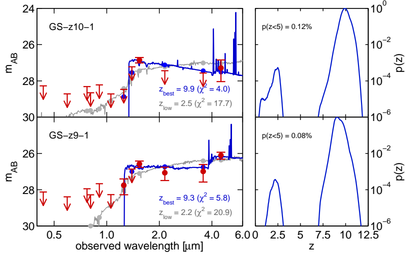
FIG. 12.— Spectral energy distribution fits (left) and redshift likelihood functions (right) for the two bright z \sim 9-10 sources in GOODS-S. In the left panel, photometry and 2\sigma upper limits are shown in dark red. Best-fit SEDs are shown as blue solid lines, in addition to the best low redshift solutions in gray. The legend lists their respective redshift and \chi^2 values. The redshift likelihood distributions from SED fitting in the right panels are shown on logarithmic axes. For both sources, the likelihood of a low redshift solution is only \sim 1\% as indicated by the labels.
