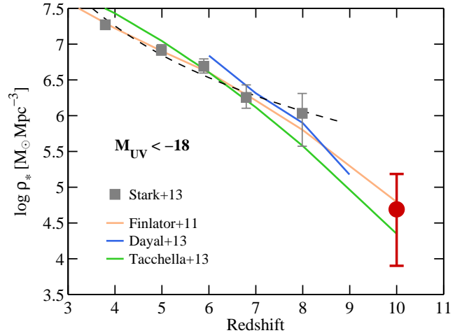
FIG. 10.— The redshift evolution of the cosmic stellar mass density in LBGs at M_{UV} \lesssim -18 to z \sim 10 . Gray squares represent the most recent determination of Stark et al. (2013), who used the measurements of González et al. (2011) and corrected these for the likely biases due to strong emission lines in the IRAC photometry for z \sim 5 - 8 sources. Their empirical trends are indicated as a dashed black line. The dark red point is our first estimate of the z \sim 10 stellar mass density based on the three GOODS-N z = 9.5 - 10.2 galaxies, the one source in GOODS-S, and the XDF candidate. For the latter, we have assumed the same M_*/L_{UV} ratio as for the average of the GOODS-N+S sources, for which these measurements can be done directly given the IRAC detections. The stellar mass density is found to be more than an order of magnitude lower at z \sim 10 than at z \sim 8 , consistent, as would be expected, with the drop in the cosmic SFR down to M_{UV} < -18 . This decrease to higher redshift is also consistent with the latest simulations and models, which are overplotted as colored lines (Finlator et al. 2011; Dayal et al. 2013; Tacchella et al. 2013). The current uncertainties on the stellar mass density measurements at z \geq 7 are still significant, however. Deeper IRAC data over larger high-redshift samples would be ideal for reducing the uncertainties in the near future.
