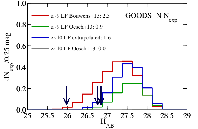
FIG. 6.— Expected number of z \sim 10 galaxy candidates per bin of 0.25 mag in the GOODS-N field for different assumptions about the UV LFs. These include previous estimates at z \sim 9 , z \sim 10 , and an extrapolation of the lower redshift UV LF trends to z \sim 10 . The total expected numbers for each assumption are indicated in the legend. The magnitudes of the three observed candidate z \sim 10 galaxies in GOODS-N are indicated by black arrows. All the tested LFs produce a distribution which peaks at significantly fainter magnitudes than observed in the sample. Furthermore, all assumed LFs result in a lower number of total expected sources at the magnitudes of the three that are observed. In particular, not a single source would be expected to be seen in GOODS-N if the estimated UV LF from the HUDF09/12 and GOODS-S fields (Oesch et al. 2013) was correct. The detection of three bright z \sim 10 candidates may thus be evidence for significant cosmic variance at the bright end of the UV LF. Such bright sources have significant consequences on the best-fit UV LF at z \sim 10 .
