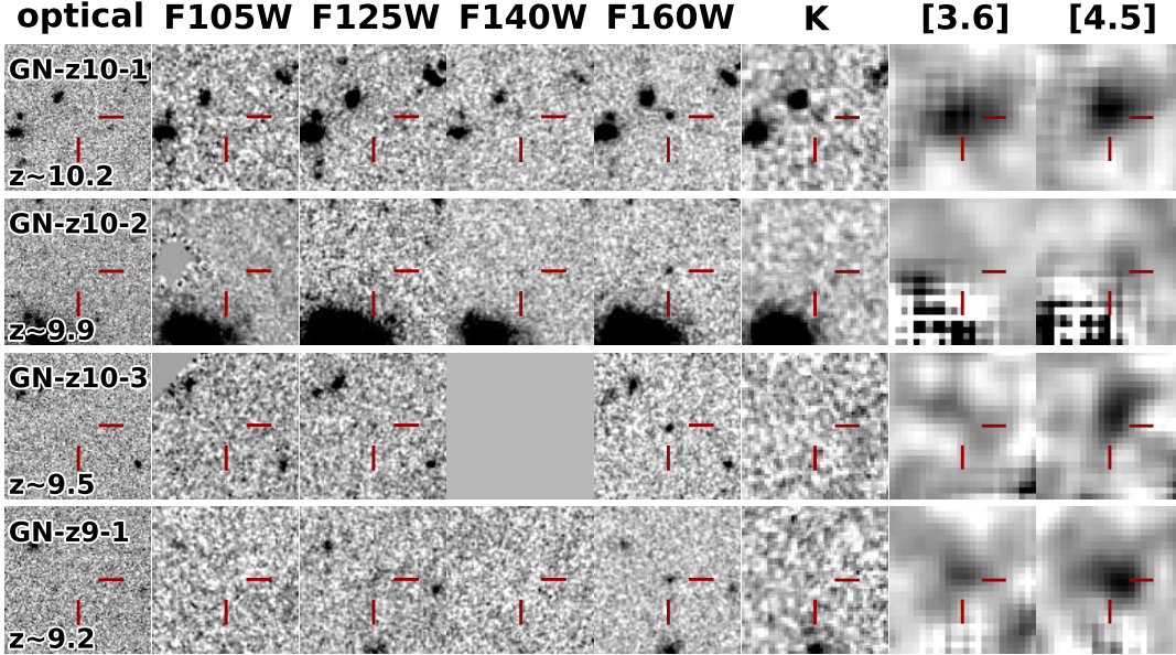
FIG. 2.— 6'' \times 6'' images of the four z \geq 9 galaxy candidates identified in the CANDELS GOODS-N data. From left to right, the images show a stack of all optical bands, Y_{105} , J_{125} , JH_{140} , H_{160} , MOIRCS K, and neighbor-subtracted IRAC 3.6 \mu\text{m} and 4.5 \mu\text{m} images. The stamps are sorted from high to lower photometric redshift from SED fits (indicated in the lower left, see also Table 2). The IRAC neighbor-subtraction works well for all sources except for GN-z10-2, where the nearby foreground source is too bright, and clear residuals are visible at the location of the candidate. Only IRAC upper limits are therefore included for this source in the following analysis. Clearly, all other sources show significant ( > 4.5\sigma ) detections in the 4.5 \mu\text{m} channel. The brightest source (GN-z10-1) is also detected at 6.9\sigma in the 3.6 \mu\text{m} channel. With the exception of the brightest candidate, which is weakly detected in the K-band (at 2\sigma ), the MOIRCS K-band data provide only upper limits.
