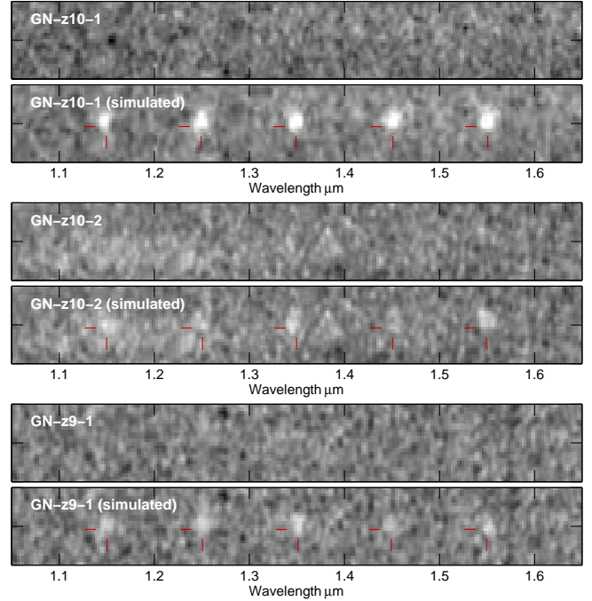
FIG. 4.— 2D WFC3/IR grism G141 spectra for the three sources for which data are available. These are GN-z10-1 (top two panels), GN-z10-2 (middle two panels) and GN-z9-1 (bottom panels) as labelled in the plots. The spectra of these sources are expected to run along the center of each panel in the horizontal direction. The spectra were smoothed slightly with a Gaussian. No significant line emission is detected for any of the three sources. Below the original data, we show a panel with a simulation of pure emission line sources at five different wavelengths, as indicated by red tick marks, with a line flux corresponding to the H_{160} photometry ( 5.5 \times 10^{-17} \text{ erg s}^{-1} \text{ cm}^{-2} for the brightest source, and 2.5 \times 10^{-17} \text{ erg s}^{-1} \text{ cm}^{-2} for the fainter two). Despite some residual contamination from a foreground source in the spectrum of GN-z10-2, such strong emission lines would have been significantly detected at > 4\sigma . The grism data rule out pure emission line source contamination for these three sources.
