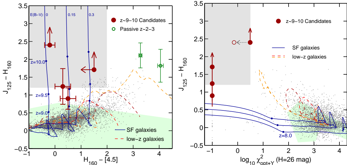
FIG. 1.— Left — The J_{125} - H_{160} vs H_{160} - [4.5] color diagram showing the location of the GOODS-N z > 9 galaxy candidates relative to other, lower redshift galaxy SED tracks. The four z \sim 9 - 10 candidates are shown with dark red circles with 1\sigma errorbars on their colors. For non-detections, 2\sigma color limits are shown. The only other sources identified as having no optical detections are shown as green circles. These two sources are very bright in IRAC, consistent with being dusty or passive sources at z \sim 2 - 3 . They are thus not included in our subsequent analysis. Also shown as small points are the locations of all sources with reliable IRAC 4.5 \mu\text{m} and H_{160} flux measurements ( > 10\sigma ) from the CANDELS GOODS-S catalog of Guo et al. (2013). These sources nicely follow the redshift tracks of evolved z < 5 SEDs (dashed yellow to red lines). The gray shaded area indicates the region in color-color space expected for z \geq 9.5 star-forming galaxies with J_{125} - H_{160} > 1.2 . Note that the initial selection of the four GOODS-N candidates was J_{125} - H_{160} > 0.5 , which selects sources at z \gtrsim 9 . The blue lines indicate the tracks of star-forming galaxies with different amounts of dust extinction ( E(B - V) = 0, 0.15, 0.3 ). Visual inspection and SED fits of the few sources from the CANDELS catalog that lie in the gray area show that they are all relatively compact, intermediate redshift, passive sources. Unlike the real high-redshift candidate sources, these are significantly detected in the optical data and so they can be clearly rejected as contaminants (see the figure to the right). The green shaded area that is well-separated from the gray selection zone indicates the area where Galactic stars are expected, including very low mass M, L, T, and Y dwarfs (see also Coe et al. 2013). Right — Plot of \chi^2_{opt+Y} (see Section 3.1) against the J_{125} - H_{160} color, representing our second selection criterion for z > 9 galaxies (which minimizes low redshift contaminants). The four z \sim 9 - 10 candidates are again shown with dark red circles, while small gray dots indicate galaxies with 10\sigma H_{160} detections in our GOODS-N CANDELS-Wide catalog. Sources with \log_{10} \chi^2_{opt+Y} < -1 are limited at that value. The shaded areas and lines represent the same as in the left panel. The \chi^2_{opt+Y} values for the SED tracks were normalized to H_{160} = 26 mag and were computed for the CANDELS-Wide field depth. The gray arrow and the open circle shows how the value of \chi^2_{opt+Y} changes for GN-z10-1 if the z_{850} -band is excluded in which a background fluctuation causes a positive 1.5\sigma flux measurement.
