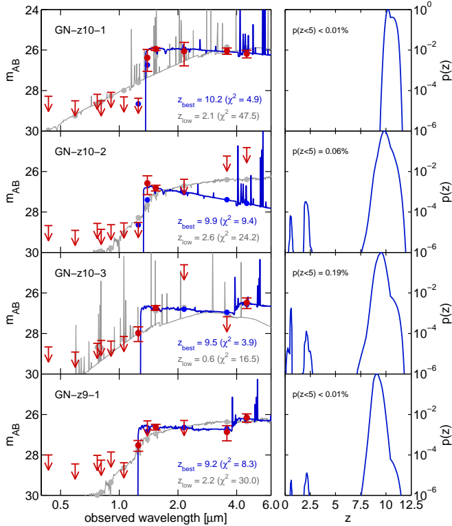
FIG. 3.— Spectral energy distribution fits to the HST and Spitzer/IRAC photometry of the four GOODS-N z \sim 9 - 10 galaxy candidates ( left ) together with the redshift likelihood functions ( right ). The measurements and their upper limits ( 2\sigma ) are shown in dark red. Best-fit SEDs are shown as blue solid lines, in addition to the best low redshift solutions in gray. The corresponding SED magnitudes are shown as filled circles. For all sources, the z \geq 9 solution fits the observed fluxes significantly better than any of the possible low-redshift SEDs. The integrated likelihoods for z_{\text{phot}} < 5 are all < 0.2\% as shown by the labels in the right panels.
