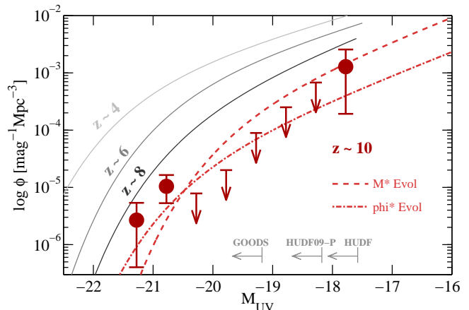
FIG. 8.— Improved constraints on the z \sim 10 UV LF from the combined z \sim 10 search using the blank-field GOODS-N, GOODS-S, and HUDF09/12/XDF WFC3/IR datasets. The additional data from fields other than the GOODS-N are taken directly from Oesch et al. (2013b). The dark red circles indicate the step-wise UV LF estimates in bins of 0.5 mag using the four GOODS-N+S and the one HUDF12/XDF z \sim 10 galaxy candidates satisfying J_{125} - H_{160} > 1.2 . Upper limits are 1\sigma . The dashed line represents the best-fit M_* -only evolution relative to the z \sim 8 UV LF, while the dot-dashed line shows the same for \phi_* -only evolution. Lower redshift LFs are shown as gray solid lines for illustration of the LF evolution trends (Bouwens et al. 2007, 2012b; McLure et al. 2013). Evolution in \phi_* appears to better match the full dataset including the new results from GOODS-N. We have not included the CLASH survey candidates (Zheng et al. 2012; Coe et al. 2013) given the uncertainties in the lensing magnification.
