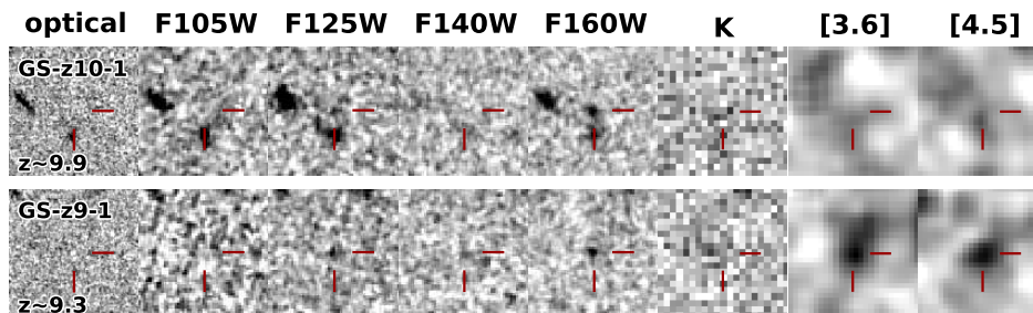
FIG. 11.— 6'' \times 6'' negative images of the two new z \geq 9 galaxy candidates identified in our re-analysis of the CANDELS GOODS-S data. From left to right, the images show a stack of all optical bands, Y_{105} , J_{125} , H_{160} , HAWKI K, and neighbor-subtracted IRAC 3.6 \mu\text{m} and 4.5 \mu\text{m} images. The K-band image is a very deep stack (26.5 mag, 5\sigma ) of ESO/VLT HAWK-I data from the HUGS survey (PI: Fontana). Both sources are only weakly detected in these data.
