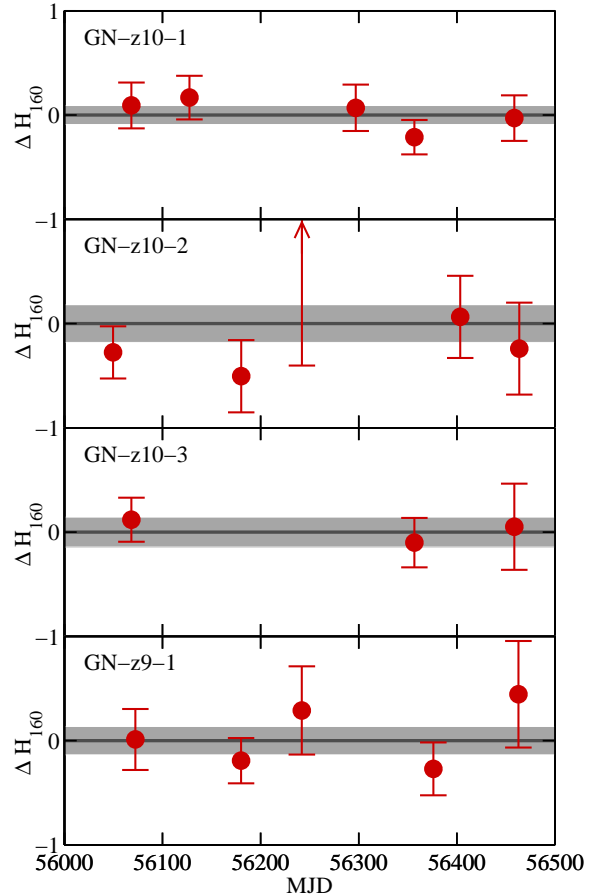
FIG. 5.— The variability of our four GOODS-N z \sim 9 - 10 candidates in the H_{160} -band. The CANDELS GOODS-N H_{160} exposures in the relevant regions were sorted by their acquisition time and binned in \sim 100 day wide bins in order to obtain five independent H_{160} images at different times. The bins were chosen as a compromise between having a significant number and having adequate S/N per bin. Given the data acquisition schedule, the times vary significantly from region to region. The figure shows the magnitude differences with 1\sigma errorbars for each source at the median acquisition time of each stack around that particular source as a function of the Modified Julian Date (MJD). Positive values correspond to fainter magnitude measurements. The gray region corresponds to the final magnitude uncertainty for each source. For almost all subsets a > 2\sigma detection is seen at the expected position. The exceptions occurred for the middle two sources. Source GN-z10-3 is in the CANDELS-Wide area and is thus covered by fewer exposures than the other sources. In two of our splits, the source landed on a masked part of the WFC3/IR detector and therefore could not be detected in those images. For GN-z10-2, we find no significant detection in the middle stack, where we show a 2\sigma upper limit on the source flux. Overall, the testing showed that there was no evidence for variability on timescales of 100 days at levels over a couple of tenths of a magnitude for any of these candidates.
