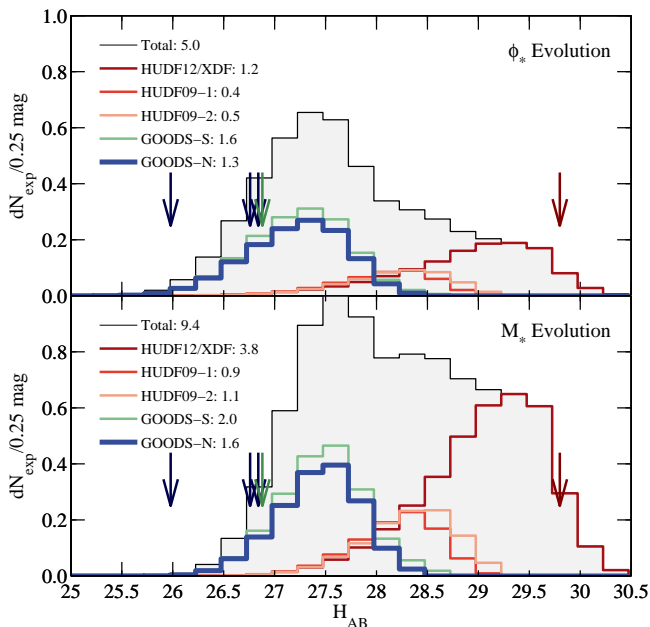
FIG. 7.— Expected number of z \sim 10 candidates per bin of 0.25 mag in the different fields used in our analysis for the best-fit UV LFs under the different assumptions of \phi_* -only (top) and M_* -only evolution (bottom). The different lines correspond to different survey fields as shown in the legend, while the shaded gray region corresponds to the total in our analysis. The legends list the breakdown of expected sources in each field for the two assumed LF evolutions. The downward pointing arrows indicate the magnitudes of the three GOODS-N z \sim 10 candidates (dark blue), the one GOODS-S source (green), and the XDF candidate (dark red). Interestingly, the detected candidates only cover the tails of the expected magnitude distribution, with no sources being detected around any of the peaks. The two assumptions result in quite different magnitude distributions and expected number of candidates in fields of different depths, which has important consequences for planning future surveys for such high-redshift sources.
