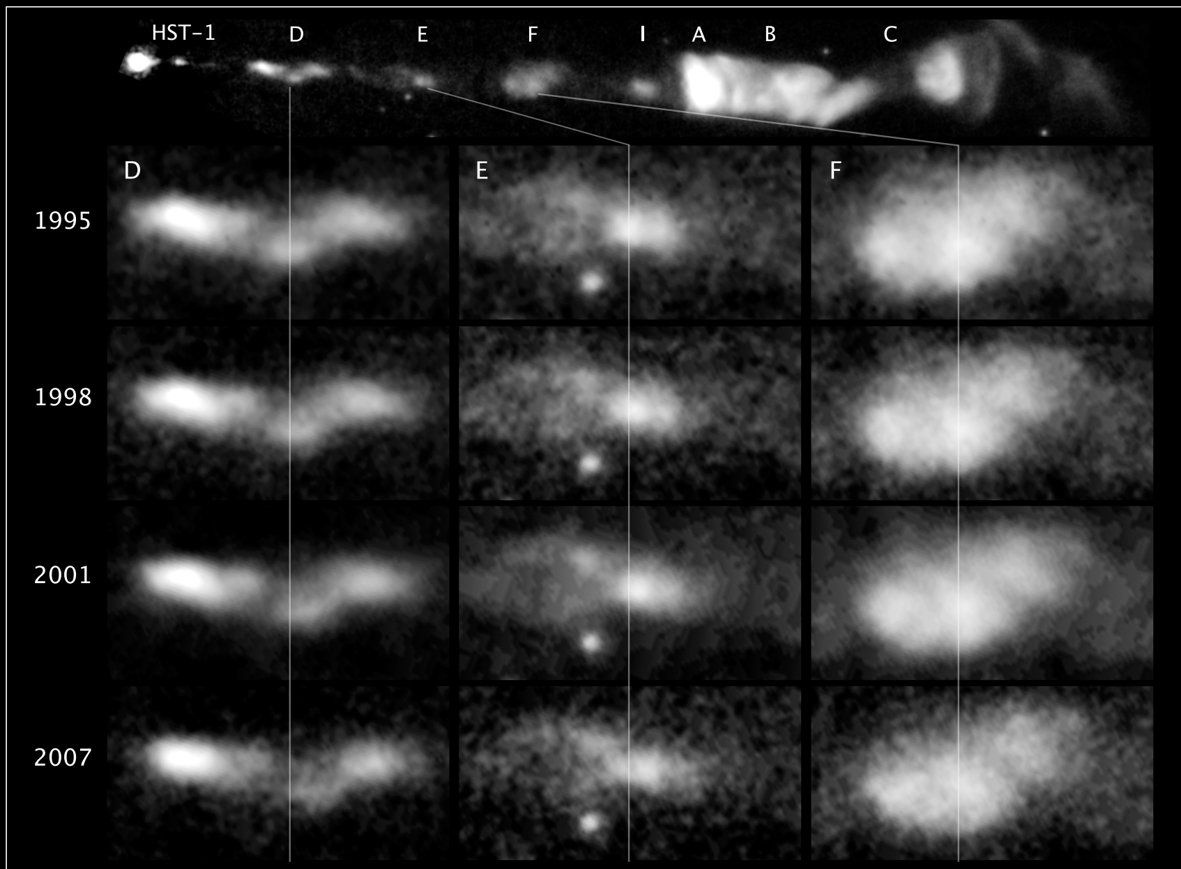
Galaxy M87 Jet Hubble Space Telescope ■ WFPC2
