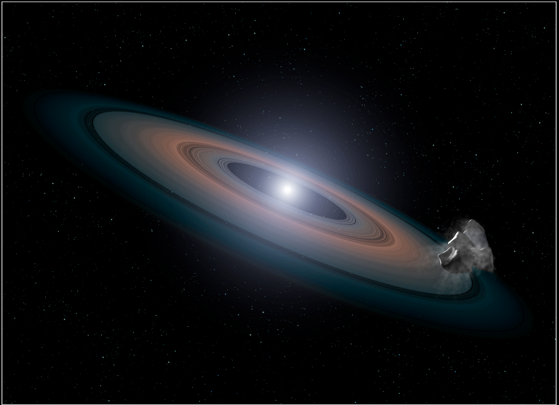
Artist's View of a White Dwarf and Circumstellar Disk
