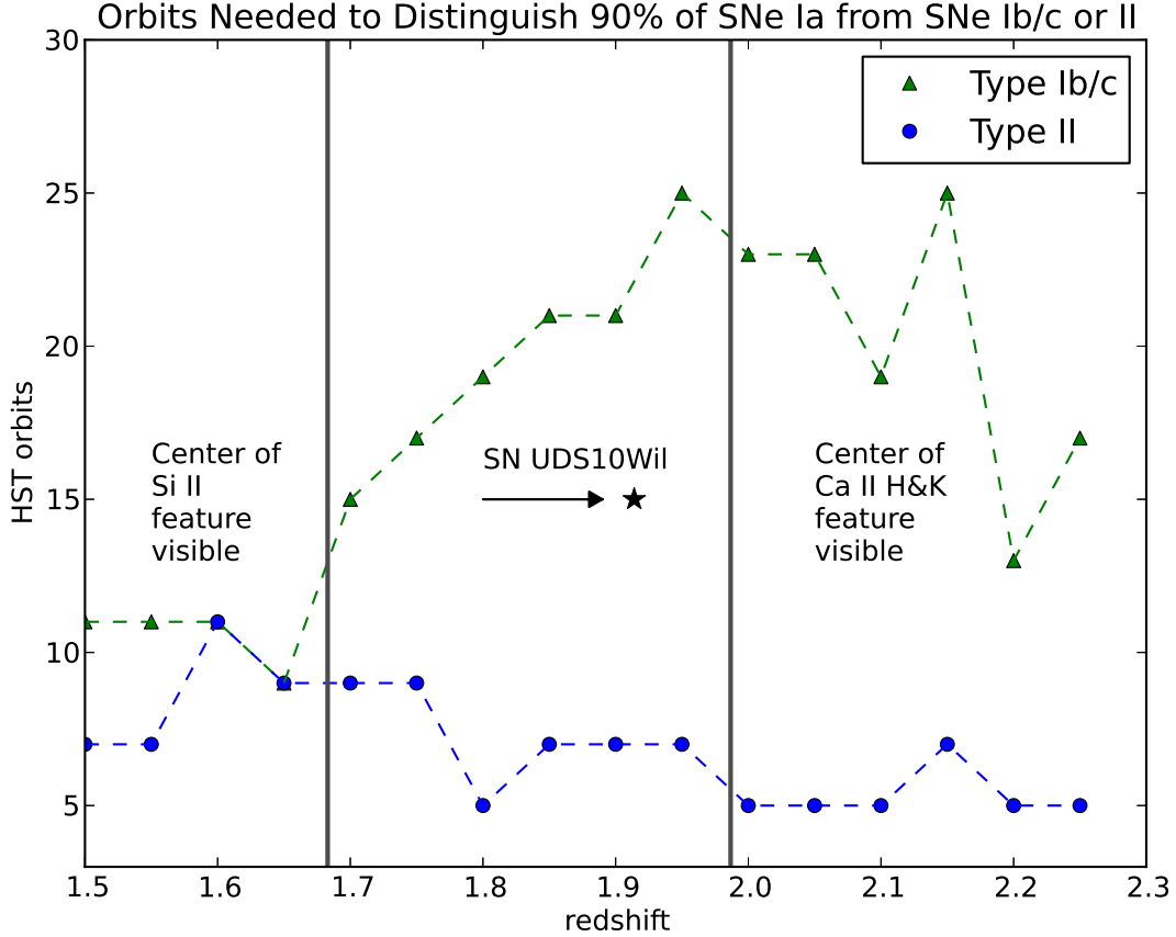
Fig. 5.— The number of orbits necessary to rule out the possibility of a SN II or SN Ib/c 90% of the time when observing a SN Ia. Using aXeSim, we simulated a variety of exposure times in the redshift range 1.5–2.3. We found that \sim 5 –10 orbits can rule out a SN II, but that the number of orbits required to rule out a SN Ib/c possibility is significantly greater. The number of orbits to rule out a SN Ib/c is much lower in the region where Si II and Ca II H&K are completely visible. These results indicate the need for photometric evidence in SN Ia classification at high redshift, although the HST grism can also be valuable in determining SN redshifts.
