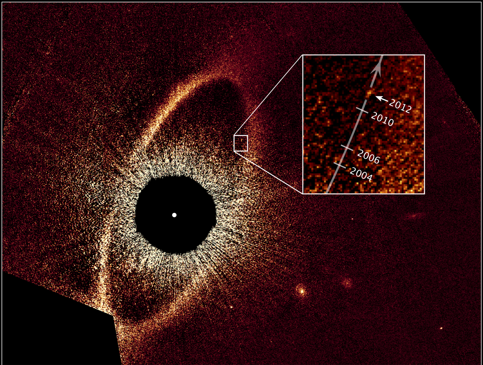
Fomalhaut System Hubble Space Telescope • STIS
