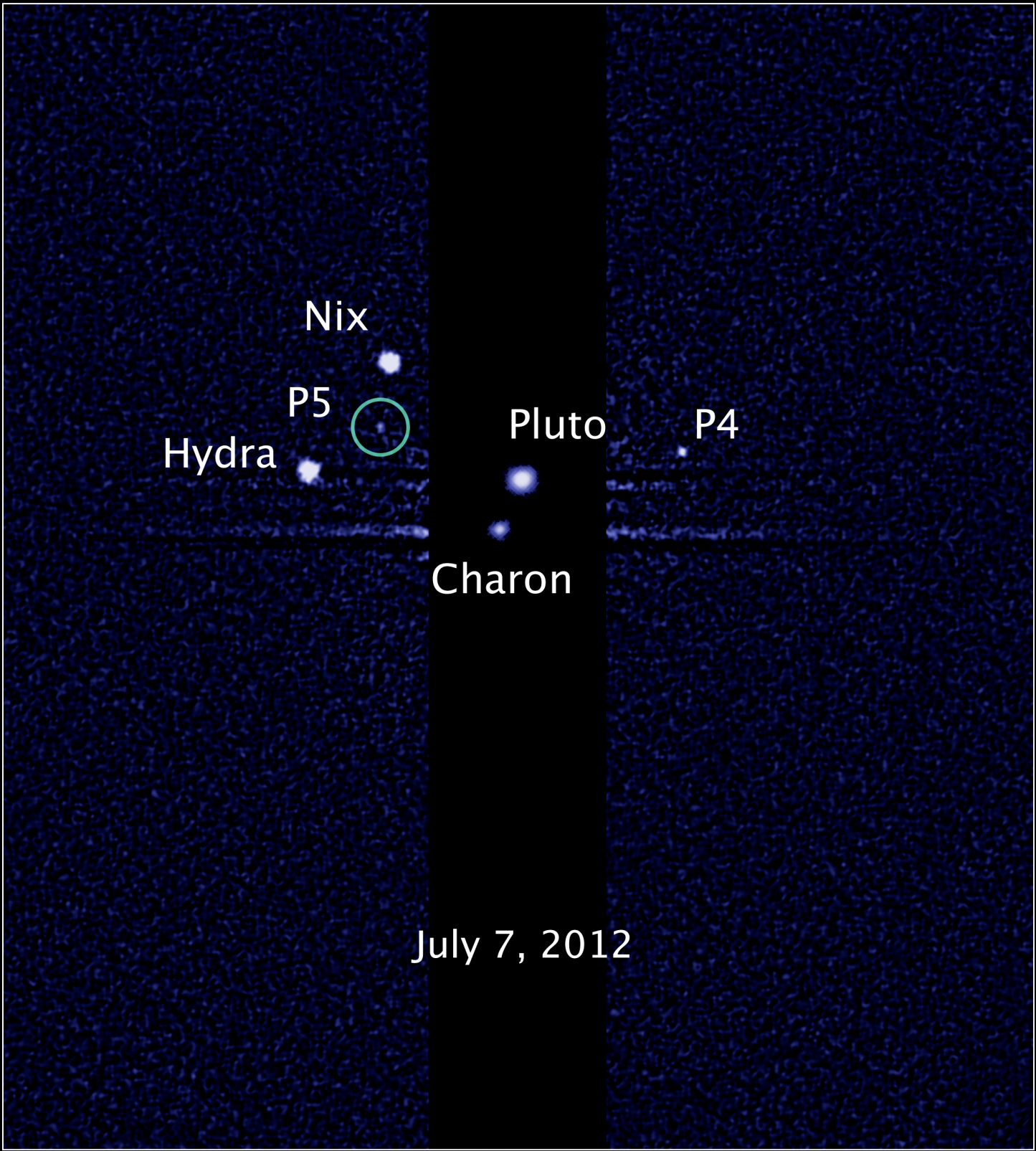
Pluto System Hubble Space Telescope • WFC3/UVIS
