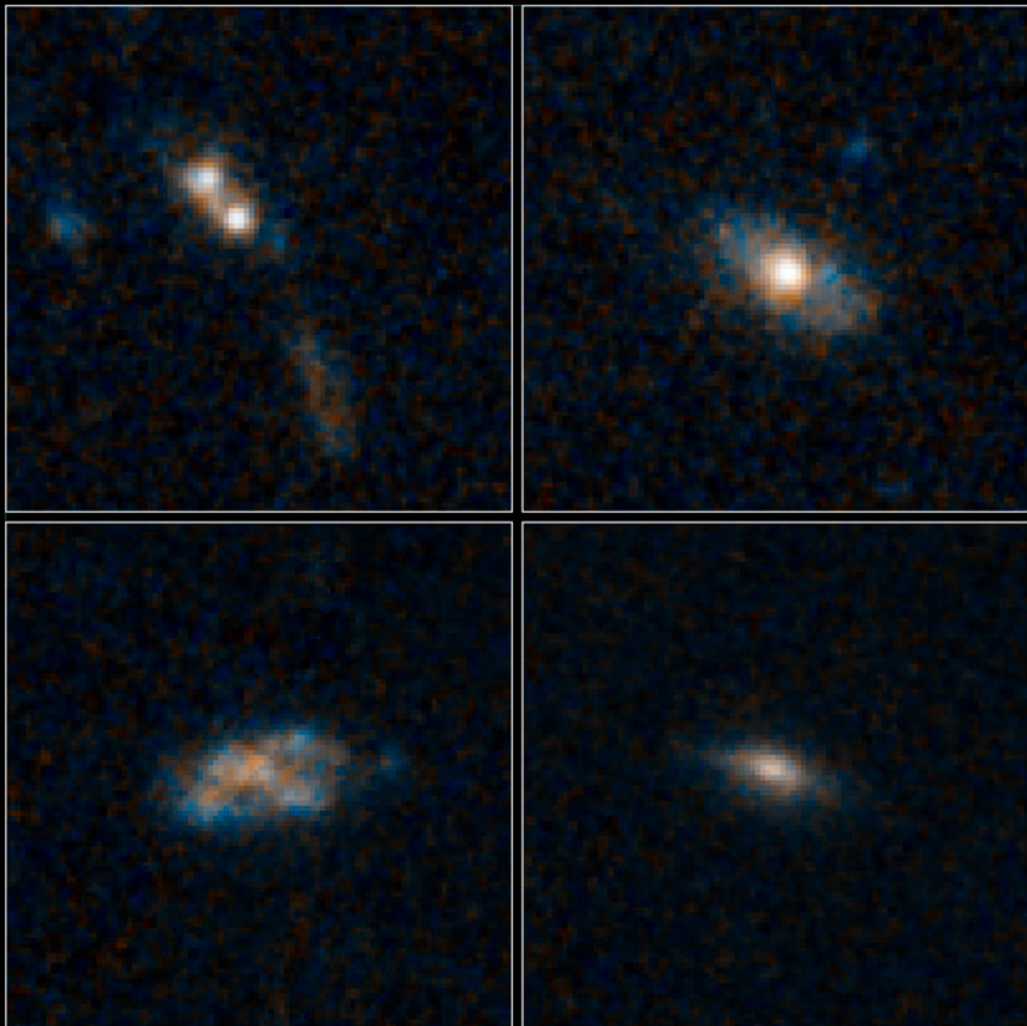
Distant, Obscured Quasars Hubble Space Telescope • WFC3/IR
