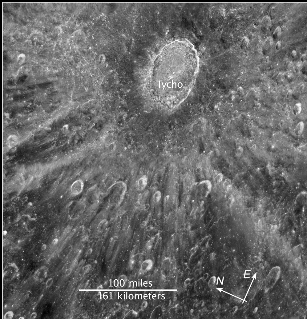
HST ACS/WFC Jan. 11, 2012
