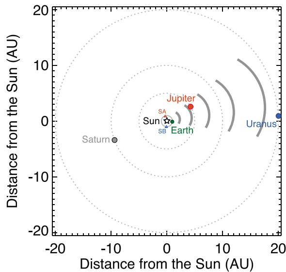
Figure 1. Planetary configuration in late 2011. A 50° wide CME propagating radially toward Uranus is shown in dark gray. SA and SB indicate STEREO A and B.
