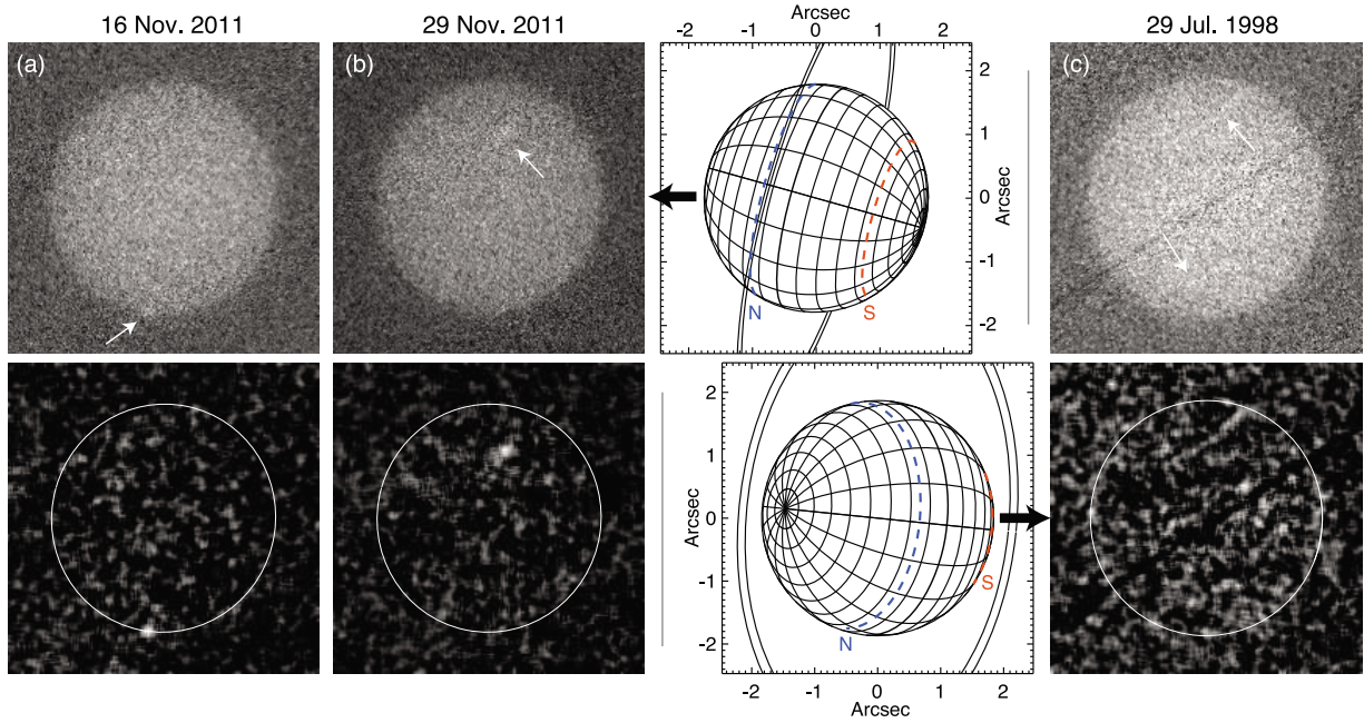
Figure 3. HST/STIS images acquired on (a) 16 Nov. 2011 15:32:10 UT, (b) 29 Nov. 2011 02:09:24 UT and (c) 29 Jul. 1998 06:07:43 UT, with the clear MAMA filter (spanning H 2 bands and H Ly- \alpha ) over 1000 s. (top) Raw images. (bottom) Same as Figure 3 (top) but after subtraction of a background of reflected sunlight and smoothing over 5 pixels (see auxiliary material). White arrows mark features of interest above the noise level: localized bright spots (Figures 3a and 3b), and north-south ring-like emissions (Figure 3c). Corresponding planetary configurations are shown with grids of planetocentric coordinates, where blue and red dashed lines indicating the latitude of the northern and southern magnetic poles.
