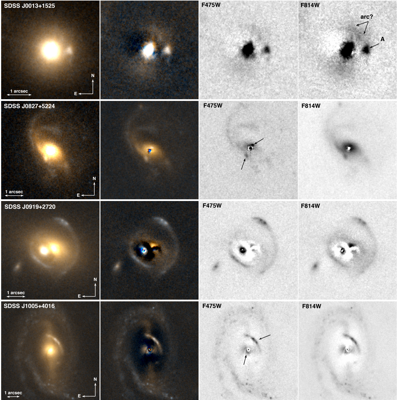
Fig. 8. HST/WFC3 images of our lensing QSOs. In each row, from left to right, we show (i) a color composite of the system, (ii) a color composite after subtraction of the QSO and of the central parts of its host galaxy, (iii) the F475W image after subtraction of the QSO and its host, (iv) the F814W image after subtraction of the QSO and its host. The arrows and labels indicate the lensed structures described in Section 7. Note that SDSS J0013+1523 was already presented in Courbin et al. (2010b) but the present HST images do not clearly support the lensing nature of this object.
