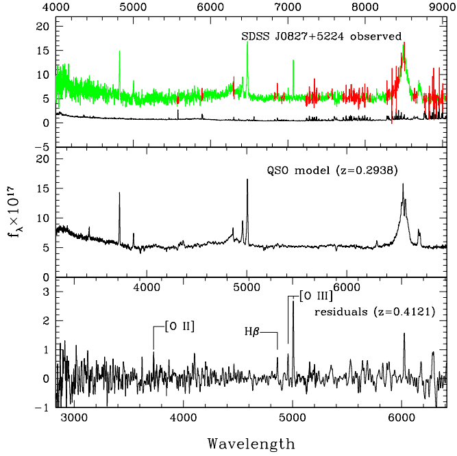
Fig. 3. Example of a spectral principal component analysis of a SDSS spectrum Top : SDSS spectrum of SDSS J0827+5224 along with the 1\sigma errors (black). The spectrum is shown in the observed frame, labeled on the upper axis. The red points are those flagged as bad in the SDSS archive, typically because of poor sky subtraction. Middle : Model of this spectrum, computed using the 43 most significant eigenspectra derived from 1000 high signal-to-noise spectra from the SDSS archive. The model is plotted against rest wavelength of the QSO, labeled below the lower boundary of this panel. Bottom : Subtraction of the model spectrum from the observed one, smoothed with a Gaussian having a full width at half maximum FWHM = 200 \text{ km s}^{-1} . The [OII], [OIII], and H\beta emission lines from the lensed object are labeled. This difference spectrum is plotted against rest wavelength in the frame of the lensed object . The significant peaks that are not labeled are all associated with regions of poor sky subtraction.
