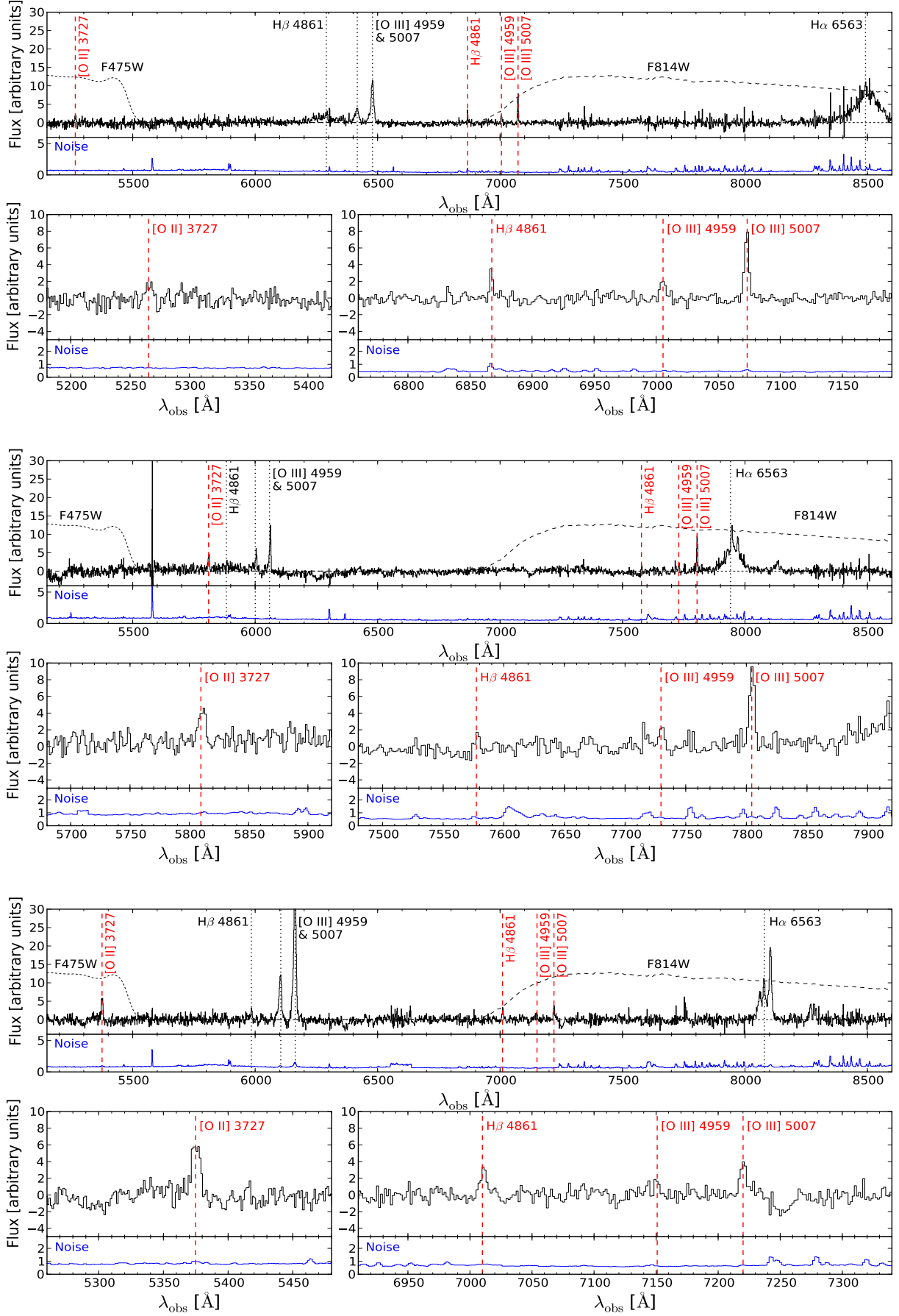
Fig. 1. SDSS spectra of the three new QSO lenses. From top to bottom are SDSS J0827+5224, SDSS J0919+2720, and SDSS J1005+4016. The emission lines of the foreground QSOs are indicated with black vertical lines (dotted) and the emission lines of the background objects are shown with red vertical lines (dashed). All three QSOs have four significant background emission lines. All spectra are shown in the observed frame. The HST filter curves are also displayed.
