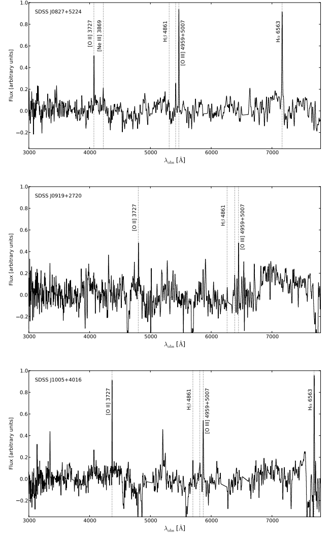
Fig. 4. PCA analysis of the Keck I spectra, shown in the observed frame. Between 3 and 6 of the emission lines of the background source are well detected depending on the object.
