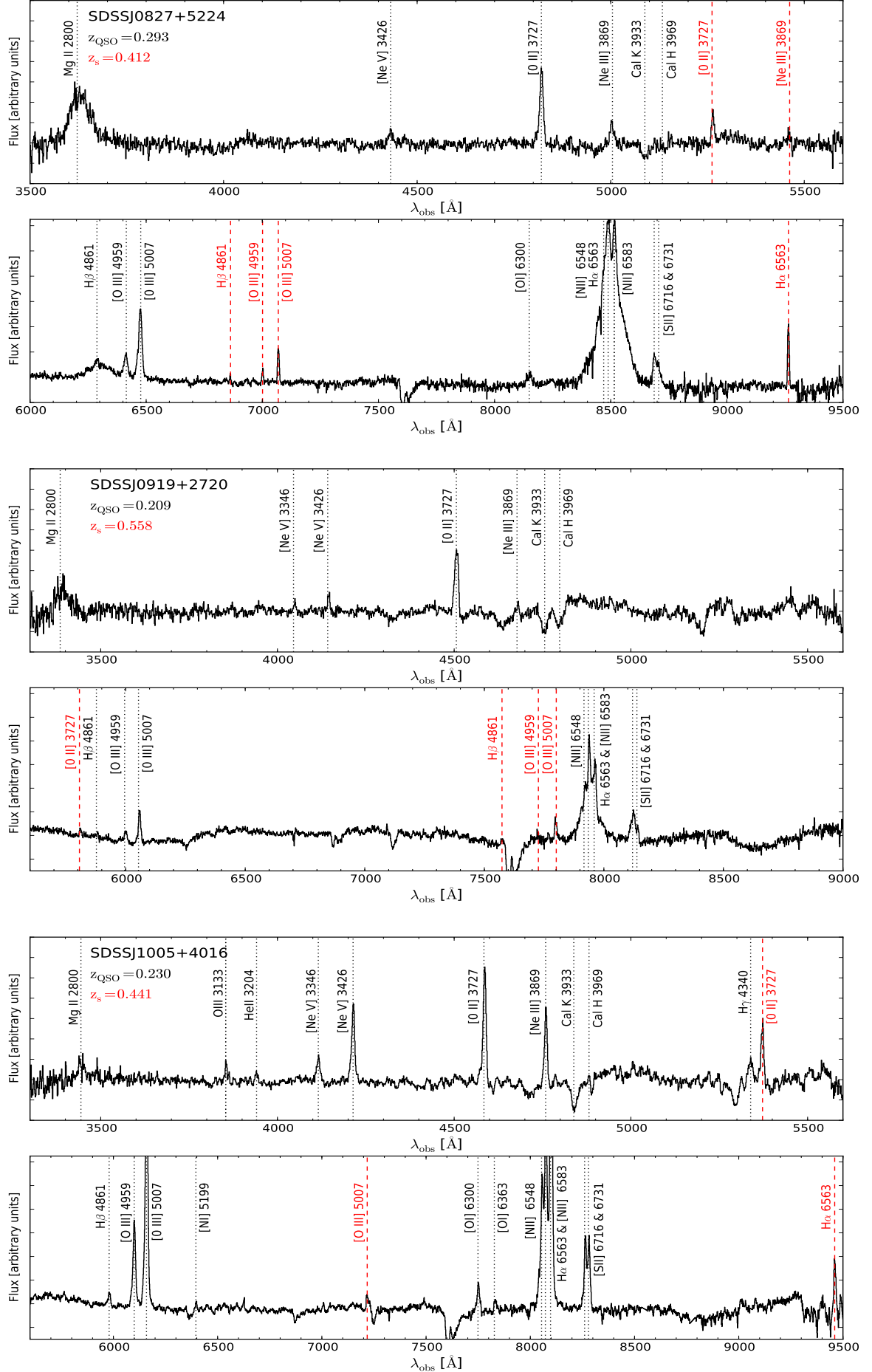
Fig. 2. Keck/LRIS spectra of the three new QSO lenses. From top to bottom are SDSS J0827+5224, SDSS J0919+2720, and SDSS J1005+4016. The emission lines are labelled as in Fig. 1. For each object the two panels correspond to the spectra obtained in the blue and red channels of the LRIS spectrograph. All spectra are shown in the observed frame. They have not been corrected for telluric absorption.
