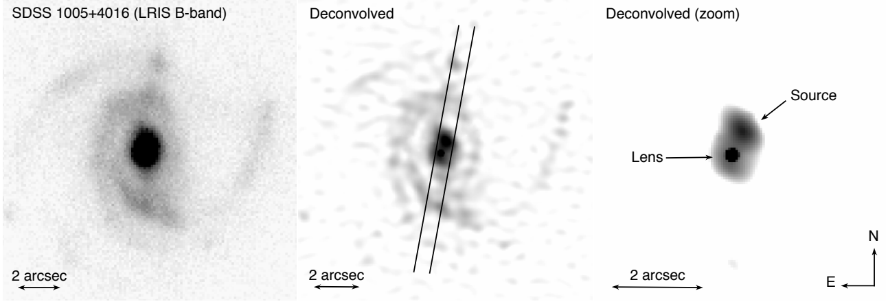
Fig. 7. Left: Keck/LRIS image of SDSS J1005+4016 ( z = 0.230 ) obtained in the B -band showing the face-on spiral QSO host galaxy. Middle: Deconvolved image showing that the nucleus of the spiral is double. The 1.5'' slit of LRIS is shown in overlay, with PA = -10^\circ . Right: Zoom of the center of the deconvolved image showing the bulge of the foreground spiral and a second object \sim 1'' to the NW.
