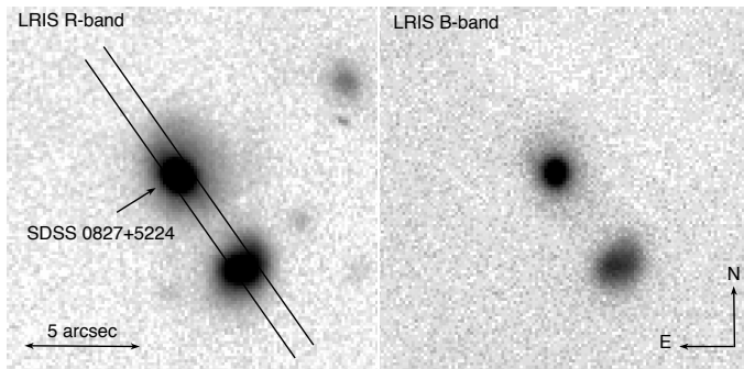
Fig. 5. Keck/LRIS images of SDSS J0827+5224 ( z = 0.293 ) in the R and B bands. The 1.5'' slit of the LRIS spectrograph is shown, oriented with PA = +30^\circ .
