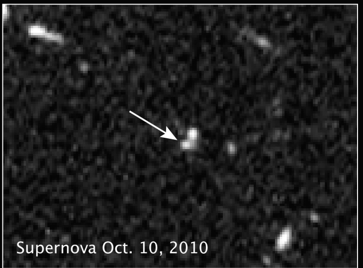
Supernova Primo in the Hubble Ultra Deep Field Hubble Space Telescope ■ WFC3 ACS
