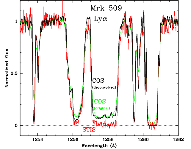
Fig. 3. Comparison of the deconvolved COS spectrum in the spectral region surrounding the \text{Ly}\alpha absorption trough (black) to the original COS spectrum (green) and the STIS spectrum (red).
