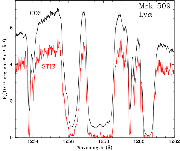
Fig. 2. COS spectrum of Mrk 509 in the \text{Ly}\alpha region (black) compared to the STIS spectrum (red).
