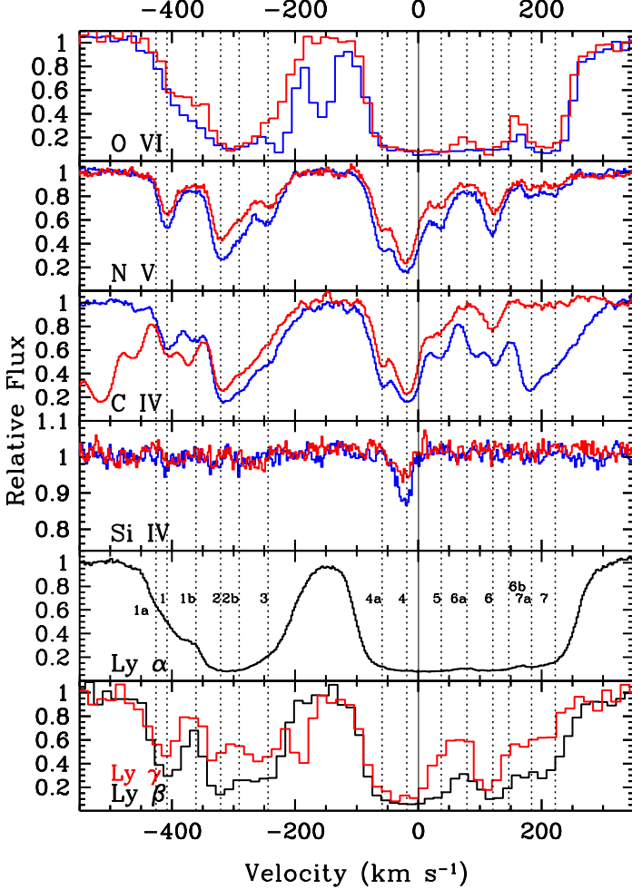
Fig. 5. Intrinsic absorption features in the COS and FUSE spectra of Mrk 509. Normalized relative fluxes are plotted as a function of velocity relative to the systemic redshift of z = 0.034397 . The top panel shows the O VI doublet from the FUSE observation in 2000 September with the red side of the doublet as a red line and the blue side of the doublet as a blue line. The middle four panels show the N V, C IV, Si IV and Ly \alpha absorption troughs from our COS observation. The bottom panel shows the Ly \gamma (red) and Ly \beta (black) absorption troughs from the FUSE observation. Dotted vertical lines indicate the velocities of identified absorption components. The thin black vertical line shows v = 0 .
