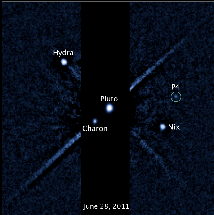
Pluto System Hubble Space Telescope ■ WFC3/UVIS
