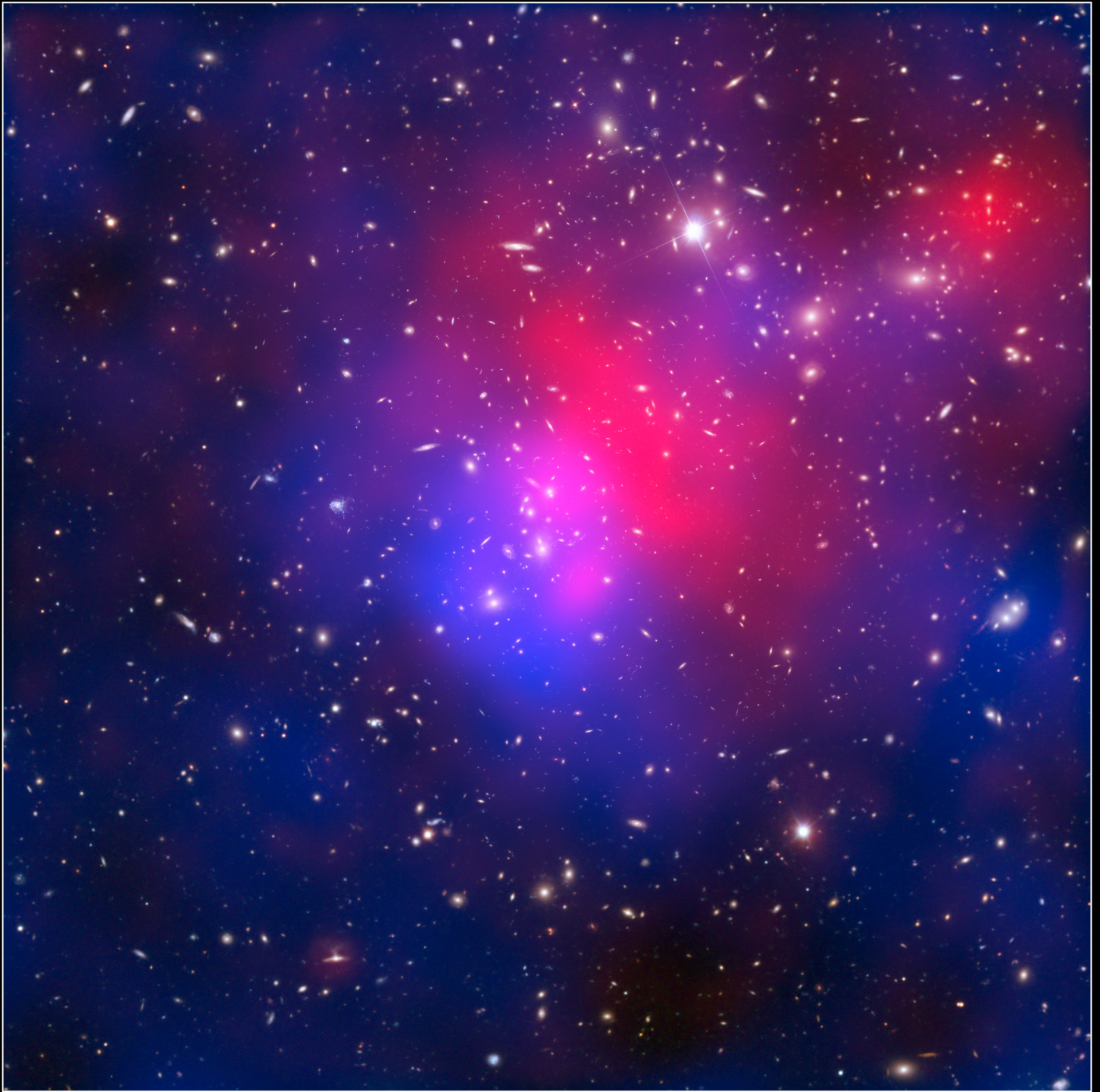
Pandora's Cluster ▪ Abell 2744 Hubble Space Telescope ACS/WFC ESO Very Large Telescope ▪ Chandra X-ray Observatory
