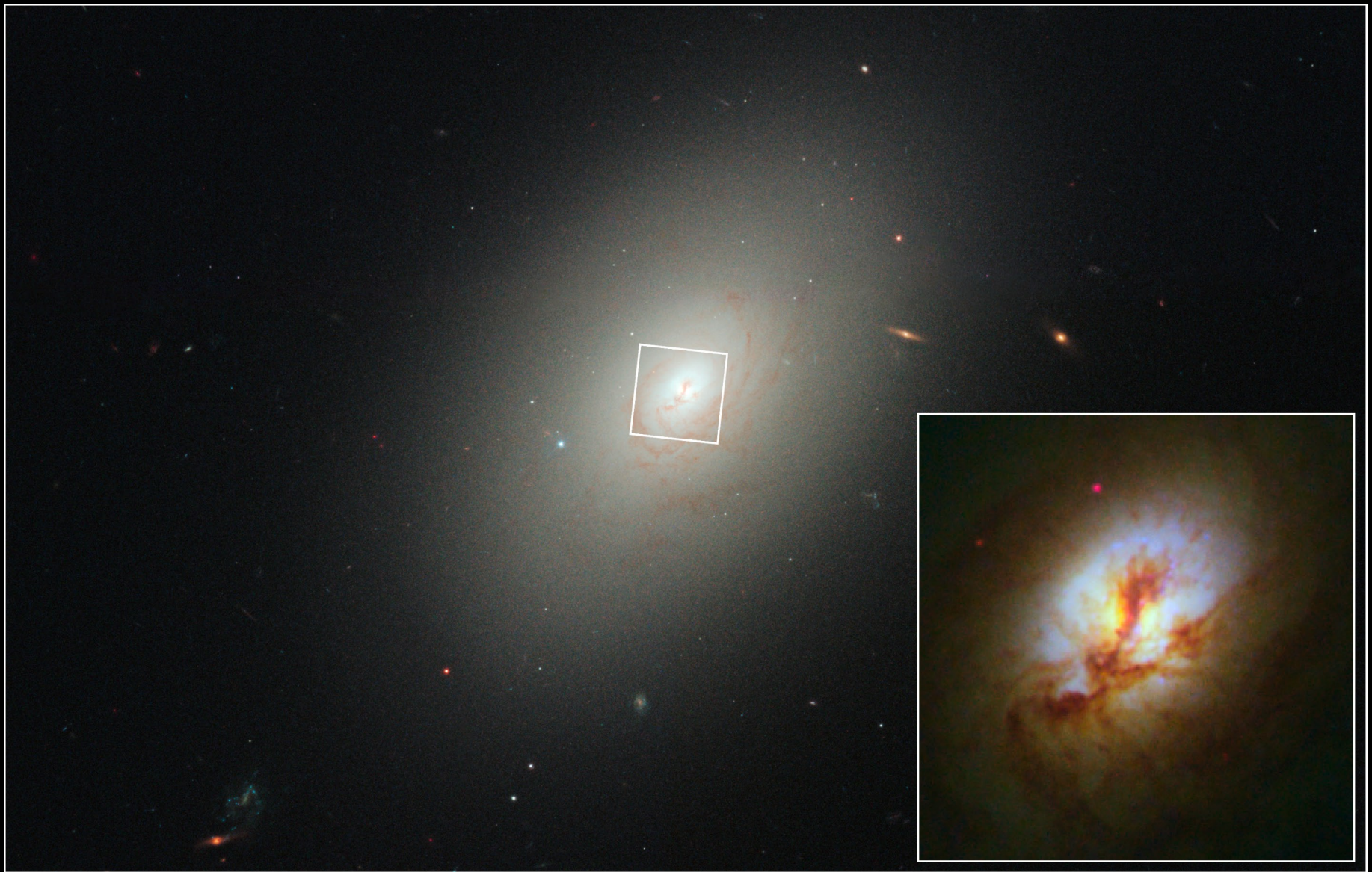
Elliptical Galaxy NGC 4150 Hubble Space Telescope WFC3/UVIS
