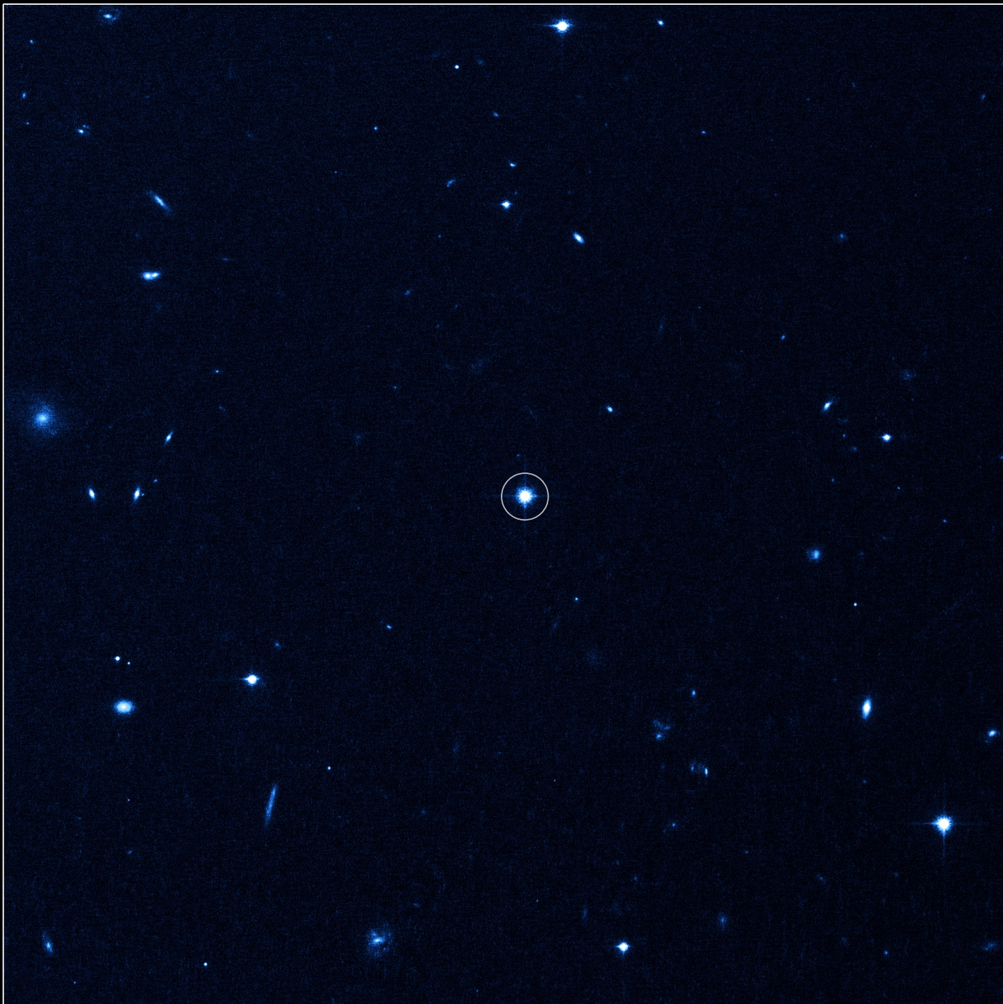
Hypervelocity Star HE 0437-5439 Hubble Space Telescope ACS/WFC
