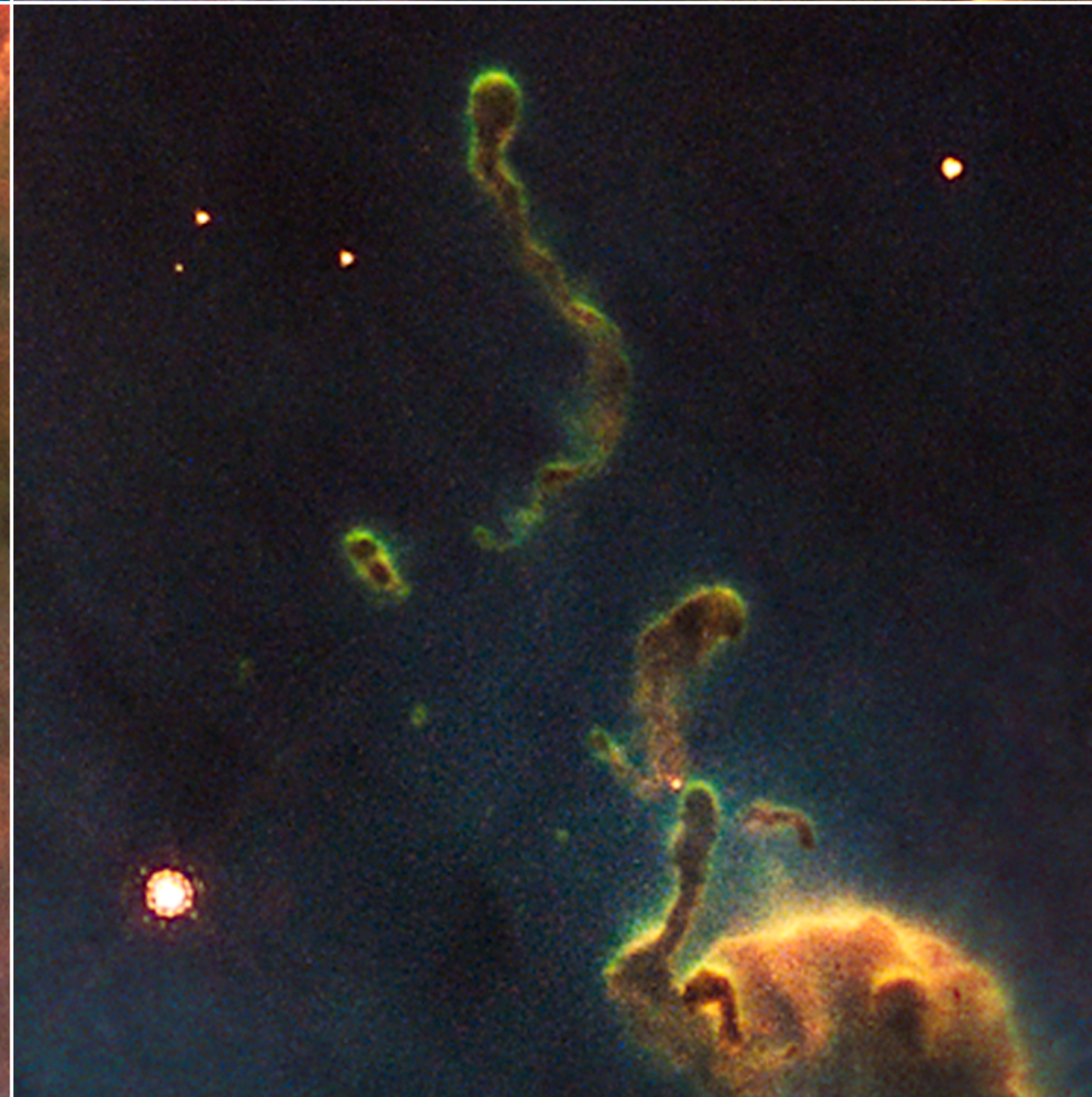
HH 901/902 Details Hubble Space Telescope • WFC3/UVIS
