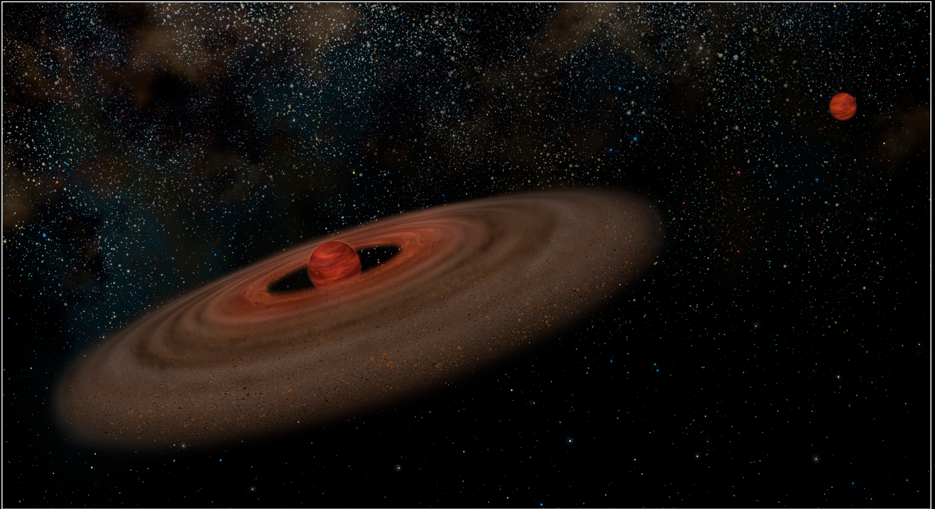
Artist's View of Binary Brown Dwarf 2M J044144 and Planetary-Mass Companion
