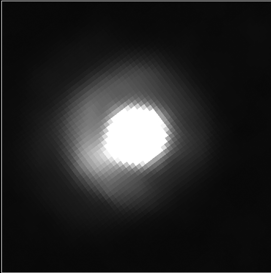
Brown Dwarf Star 2MASS J044144 and Planetary-Mass Companion Hubble Space Telescope • WFPC2
