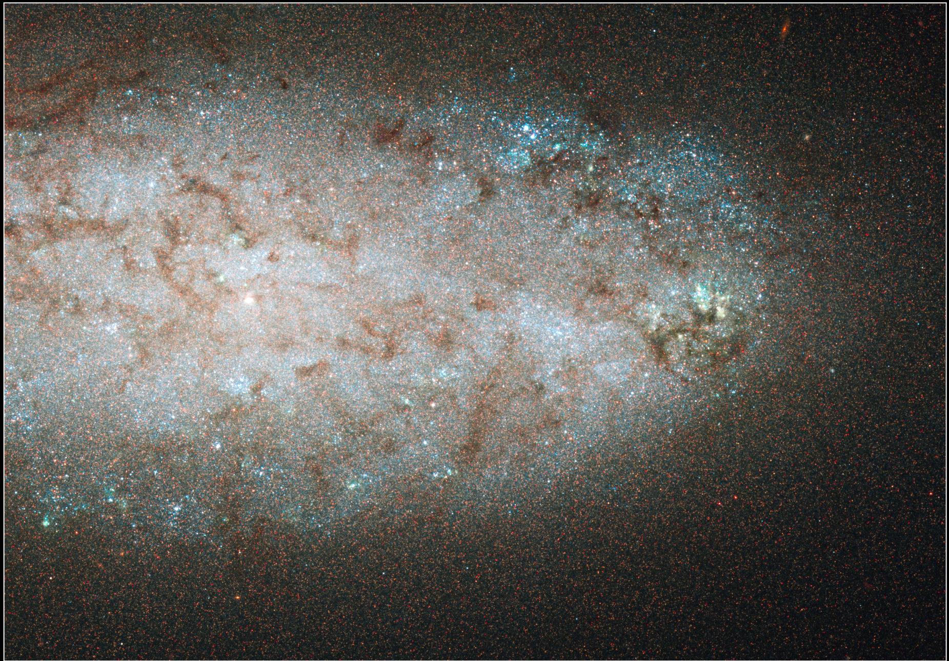
Spiral Galaxy NGC 2976 Hubble Space Telescope • ACS/WFC
