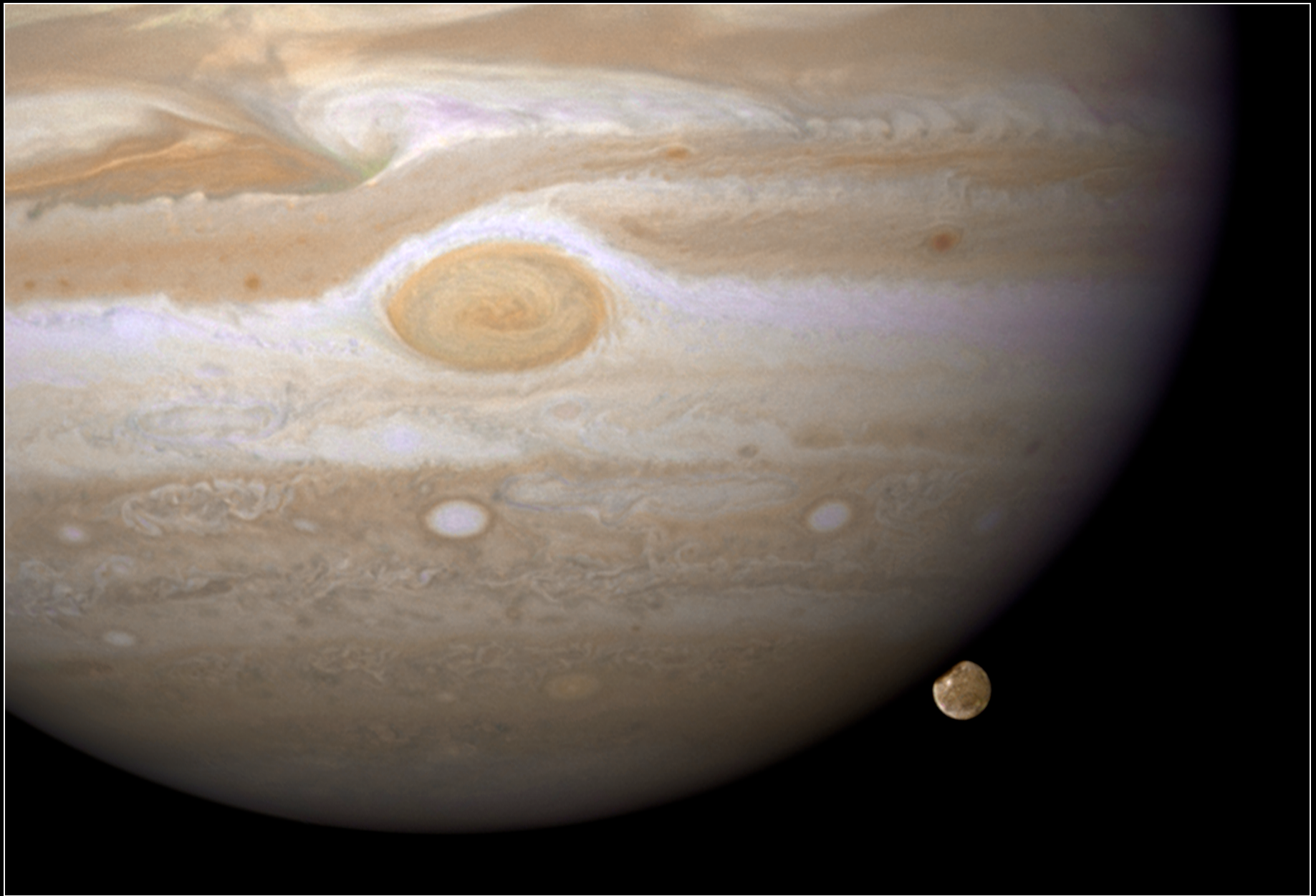
Jupiter and Ganymede • April 9, 2007 Hubble Space Telescope • WFPC2
