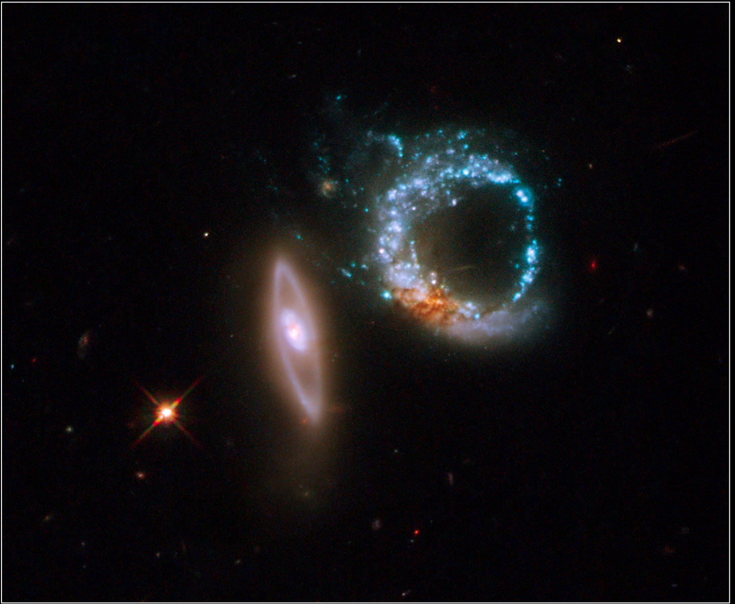
Interacting Galaxies Arp 147 Hubble Space Telescope • WFPC2
