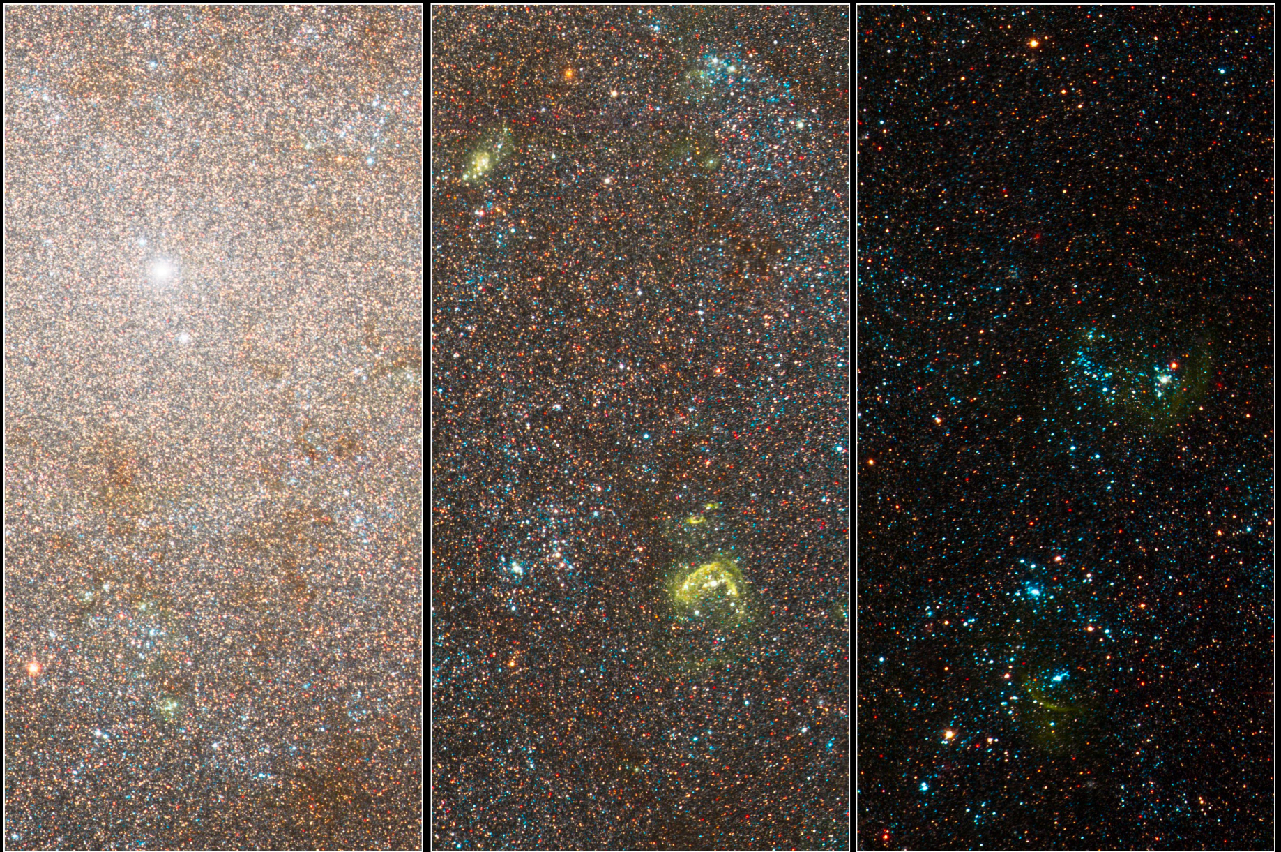
Spiral Galaxy NGC 300 • ANGST Hubble Space Telescope • ACS/WFC
