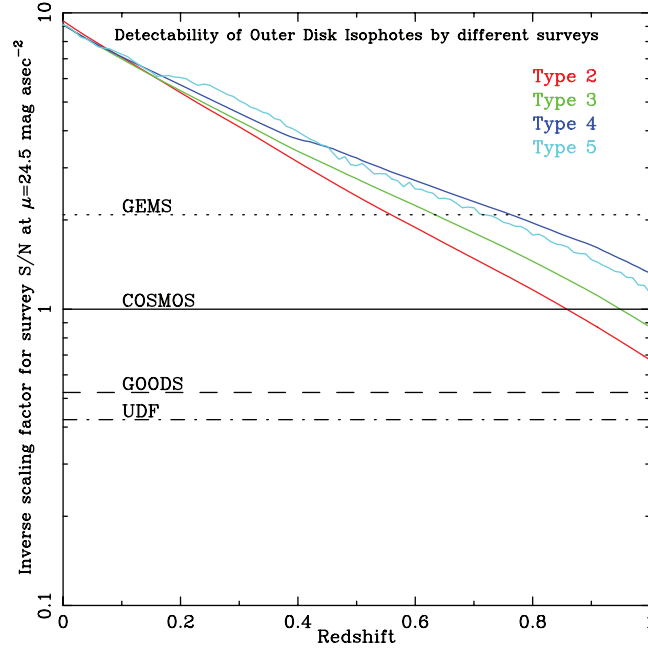
FIG. 10.— Plot of the noise-to-signal ratio for 0.6'' diameter galaxy with a rest-frame \mu_{LB} = 24.5 \text{ mag arcsec}^{-2} in COSMOS. The choice of 0.6'' diameter was based on previous studies of galaxy sizes (Ferguson et al. 2004). Our own data are consistent with these size estimates. We find that the median exponential scale length of L^* galaxies in COSMOS is 3.1 \text{ kpc} ( 0.39'' ) at z = 0.835 (Sheth et al. 2008). In the sample analyzed here, 93% of the galaxies have a half-light radius greater than 0.3'' . So the noise to signal measurement shown here for COSMOS data for the outermost disk isophote is a lower limit. The horizontal lines show the 1 \sigma sensitivity limits for the COSMOS, GEMS, GOODS, and UDF survey. Note that GEMS will be adversely affected in measurements f_{\text{bar}} even for L^* galaxies at z > 0.5 because of the low signal-to-noise ratio in the underlying disk.
