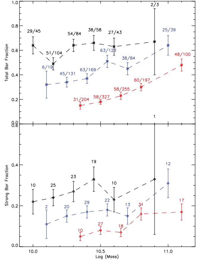
FIG. 3.— Total bar fraction ( top panel ) and strong bar fraction ( bottom panel ) vs. total galaxy stellar mass in three redshift bins. As expected from Fig. 2, there is a strong correlation between the bar fraction and the mass for the highest redshift bin. In that bin, galaxies with \log M > 10.9 already have f_{\text{bar}} \sim 0.5 , whereas galaxies with \log M < 10.5 have f_{\text{bar}} < 0.2 . The bar fraction for the entire population evolves with time with the largest change in the lowest mass bin. The same trend is seen in the bottom panel. The lack of high-mass galaxies in the lower redshift bins is because, even with 2 \text{ deg}^2 , the volume of space observed by COSMOS is small. Luminosity and color selection criteria put a limit on the minimum detectable mass—our sample is complete for the points shown here. Each point is at the left edge of bins of \delta \log M = 0.15 , starting from 10.0 (point skipped if no data is found in a bin). Errors bars are calculated as before and last bin is from \log M = 10.9 – 11.5 . The data points are slightly offset along the x-axis for each redshift bin and only the number of strong bars is labeled on the bottom panel for clarity. The uncertainty in the mass measurement is a factor of three. This figure should be viewed together with Fig. 2.
