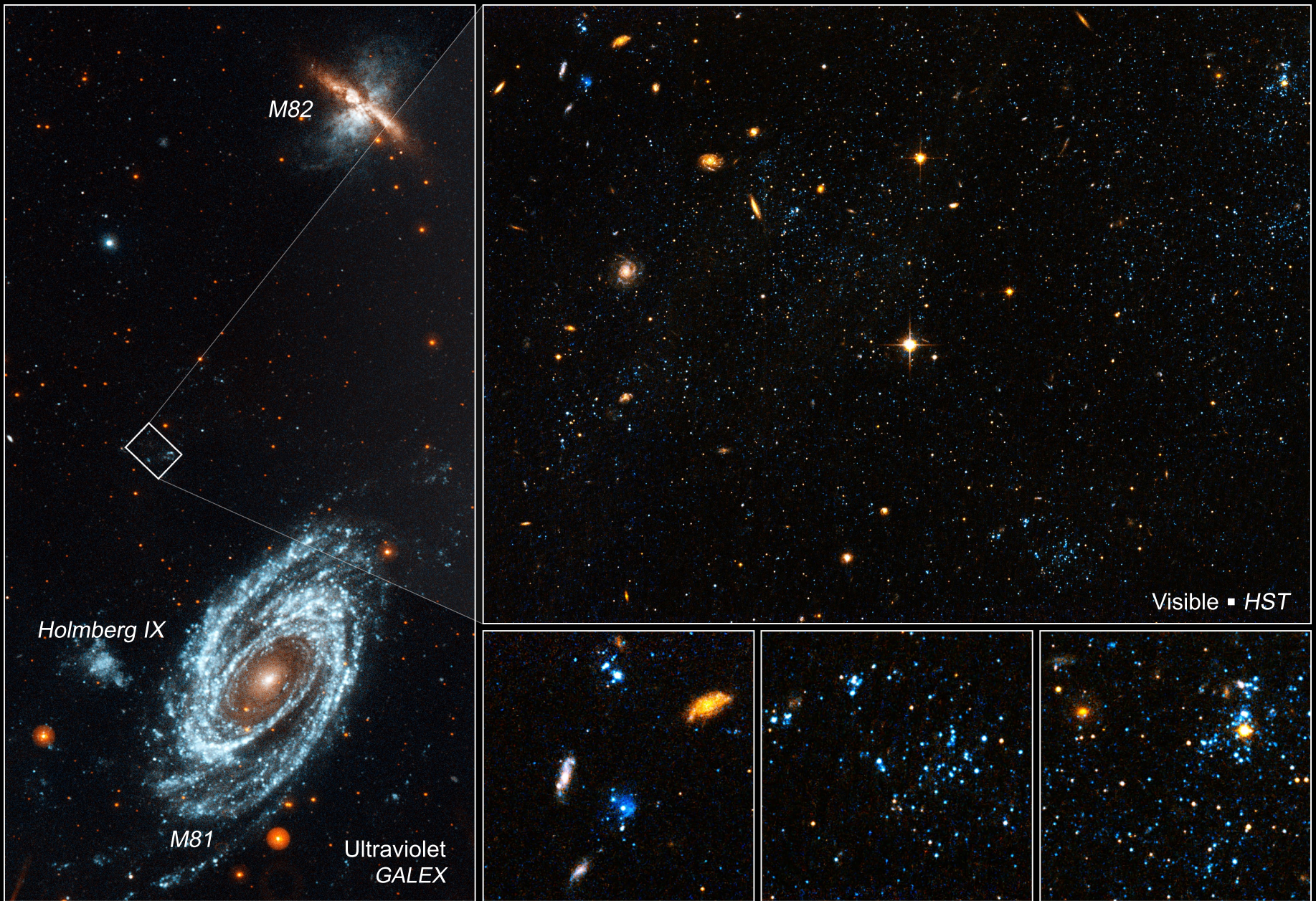
Arp's Loop in the M81–M82 Galaxy Group Hubble Space Telescope ■ ACS/WFC
